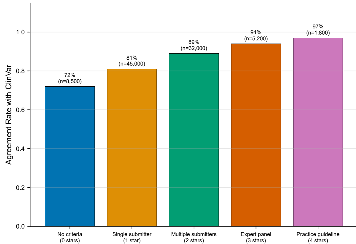
(a) Agreement vs. ClinVar Review Confidence
