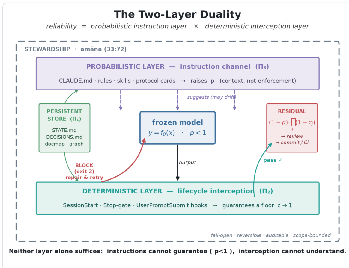
Figure 1. The two-layer duality. The probabilistic instruction layer ( \Pi_3 , purple) raises p by loading context but may drift (dashed arrows); the deterministic interception layer ( \Pi_2 , teal) executes regardless of the model's choice and either passes the turn or blocks it (exit 2) back into the model for repair. The persistent store ( \Pi_1 ) feeds both. What escapes both layers is the residual (1-p) \cdot \prod_j (1-c_j) , handed to review or a later commit/CI gate. The whole sits inside a stewardship boundary (amāna, §9). Neither layer alone suffices — the formal content of the discipline never trust the output; earn trust with a check .
