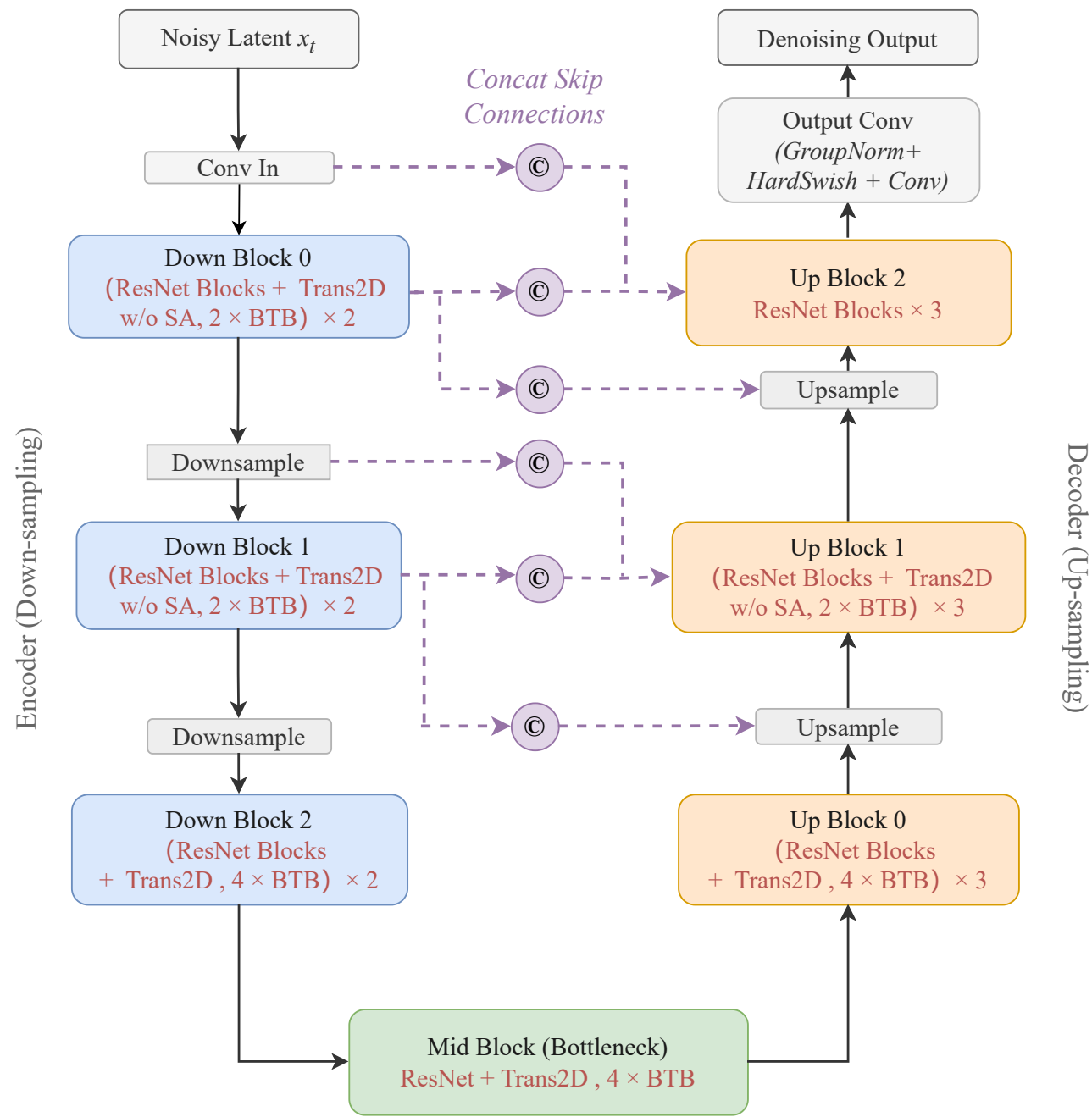
(a) Denoiser Architecture
