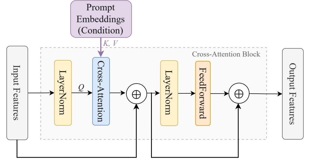
(e) Basic TransformerBlock w/o SA
