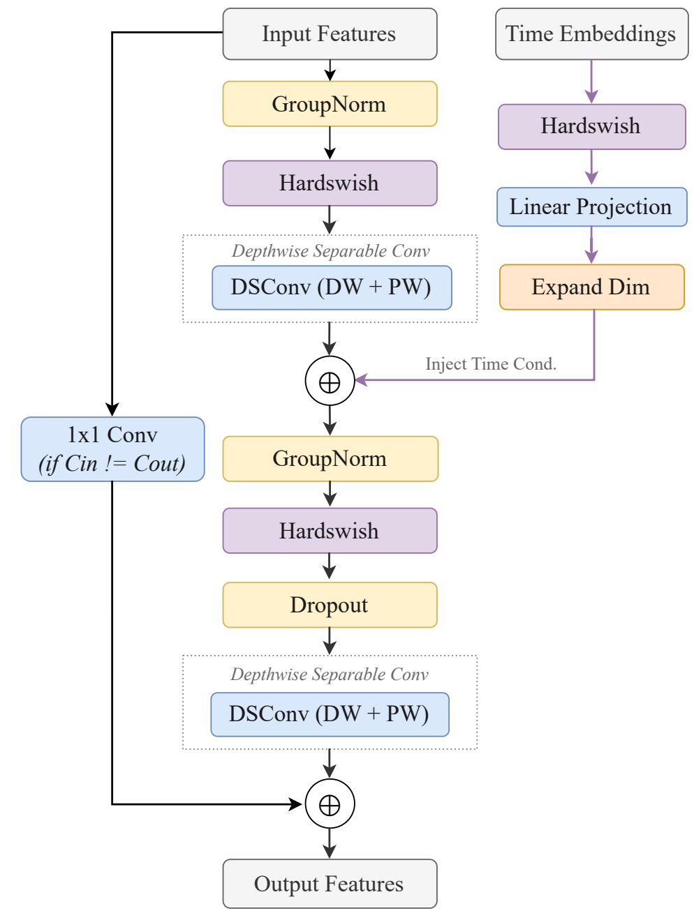
(c) ResNet Block
