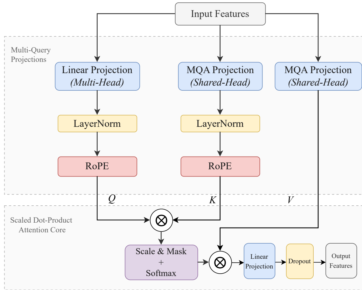
(b) Self-Attention
