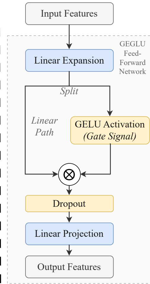
(c) FeedForward
