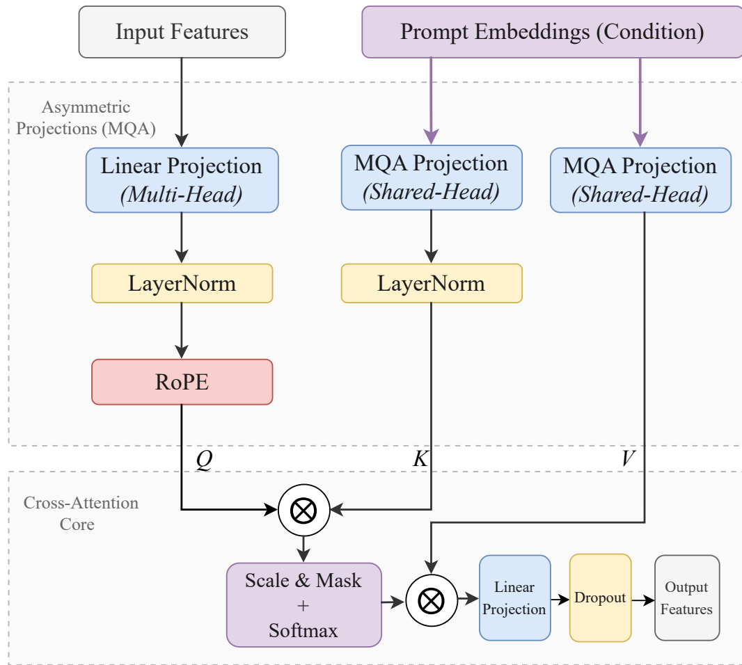
(a) Cross-Attention
