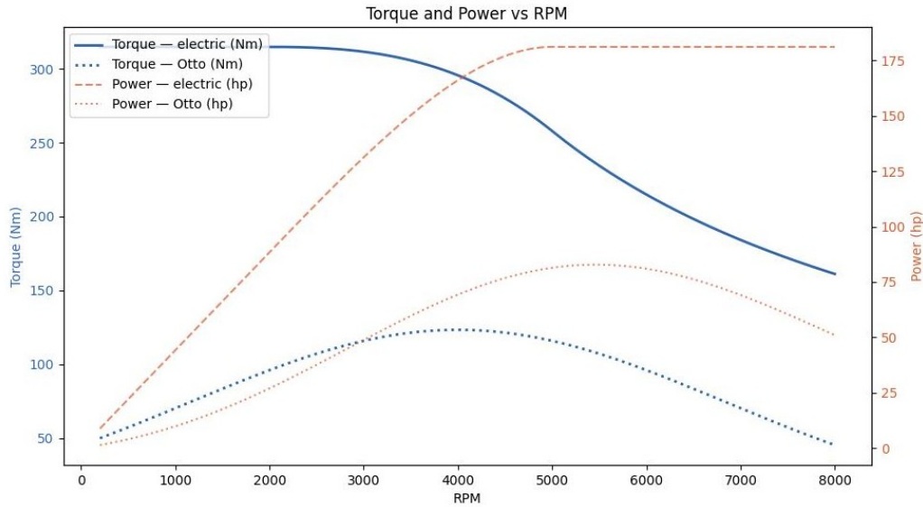
Figure 5 Torque-Power plot for hybrid vehicle combined power plant.
