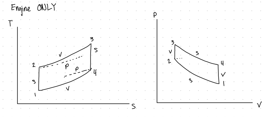
Figure 2 The T-s and P-v Diagrams of the Otto Engine
