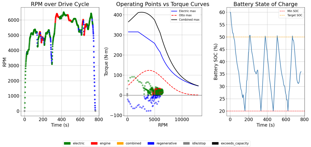
Figure 7 Results for Highway Driving Schedule
