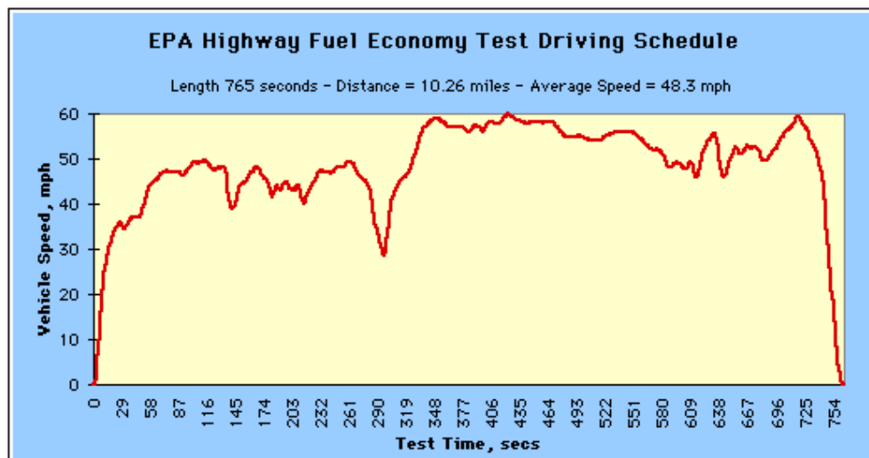
Figure 9 EPA Highway Dynamometer Driving Schedule
