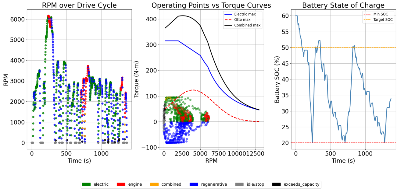
Figure 6 Results for Urban Driving Schedule
