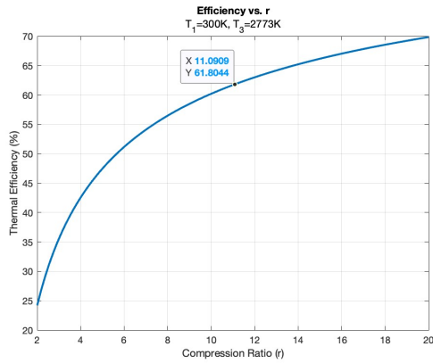
(a) Thermal Efficiency of Otto Cycle Vs. Compression Ratio.
