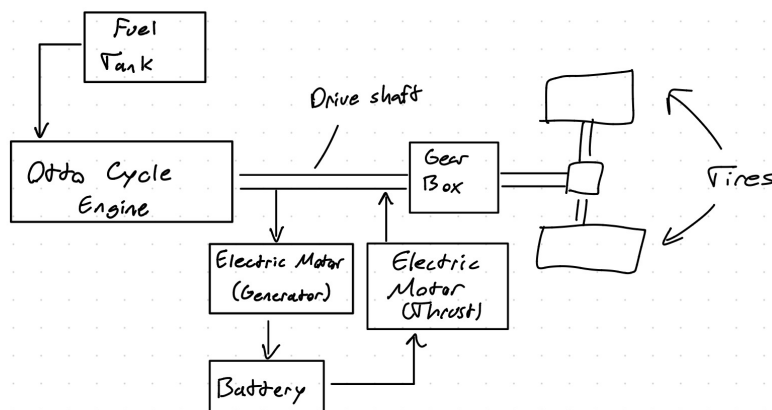
Figure 3 Block Diagram of a series-parallel configuration for a hybrid car powertrain.
