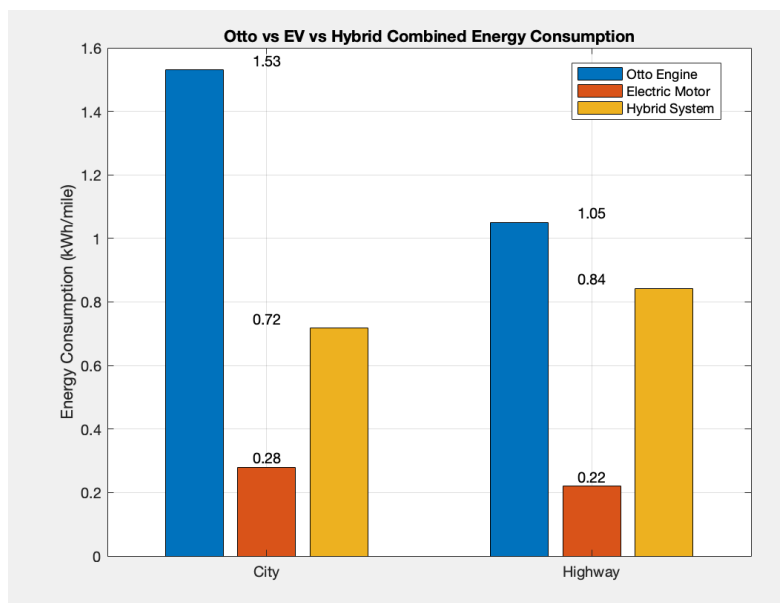
Figure 1 Energy Consumption of Otto vs. Electric vs. Hybrid
