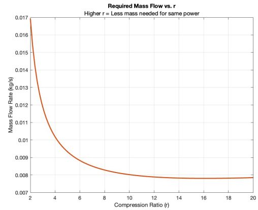
(b) Mass Flow Rate Vs. Compression Ratio
