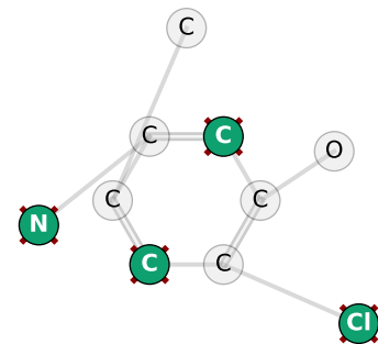
e Reactivity
