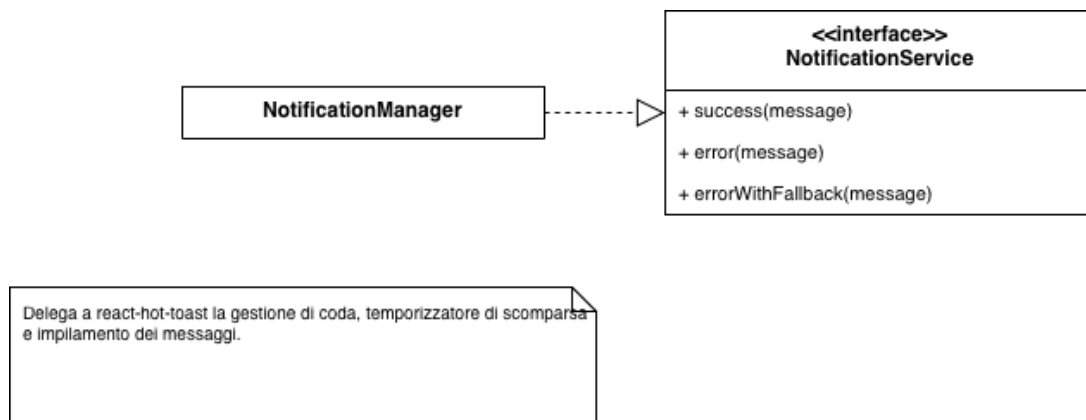
Figura 12: NotificationManager: classe infrastructure
