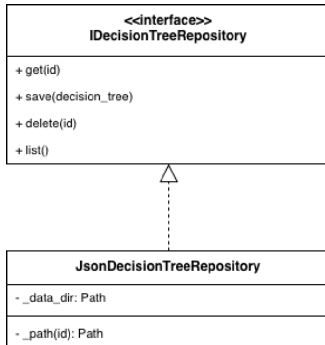
Figura 22: JsonDecisionTreeRepository: classe persistence
