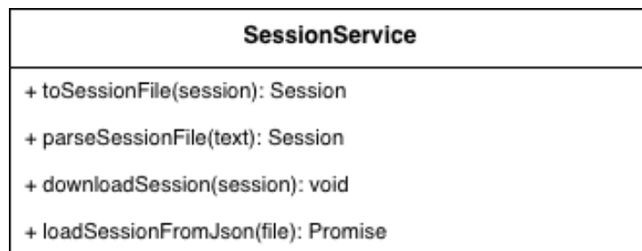
Figura 5: SessionService: modulo application
