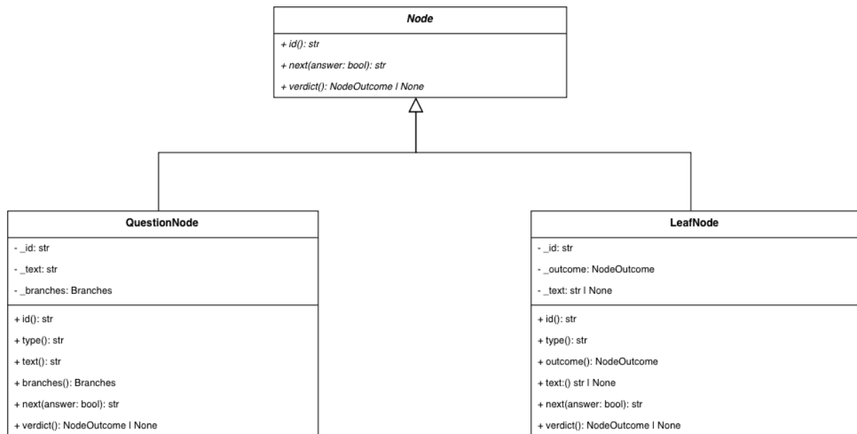
Figura 31: Node: classe backend G
