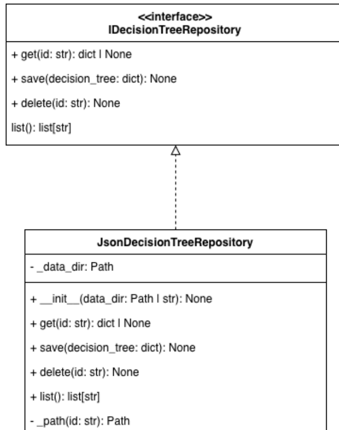
Figura 21: IDecisionTreeRepository: interfaccia G persistence
