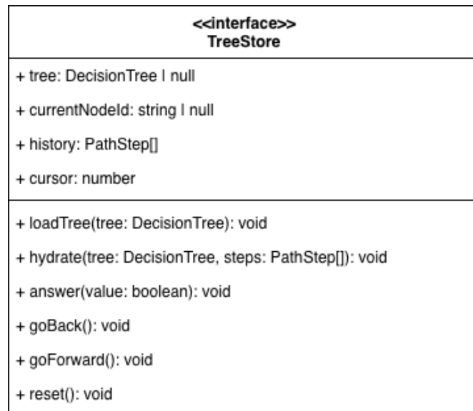
Figura 17: TreeStore: Store state management
