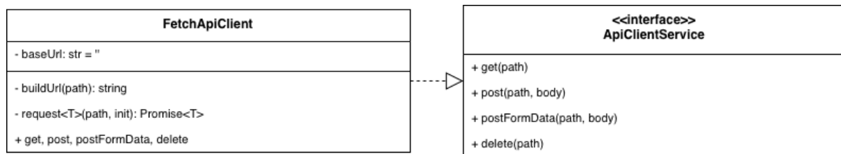
Figura 9: FetchApiClient: classe infrastructure
