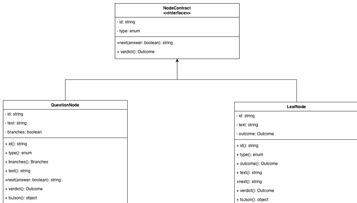
Figura 26: Node, QuestionNode e LeafNode: classe frontend G
