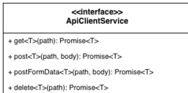
Figura 8: ApiClientService: interfaccia G infrastructure
