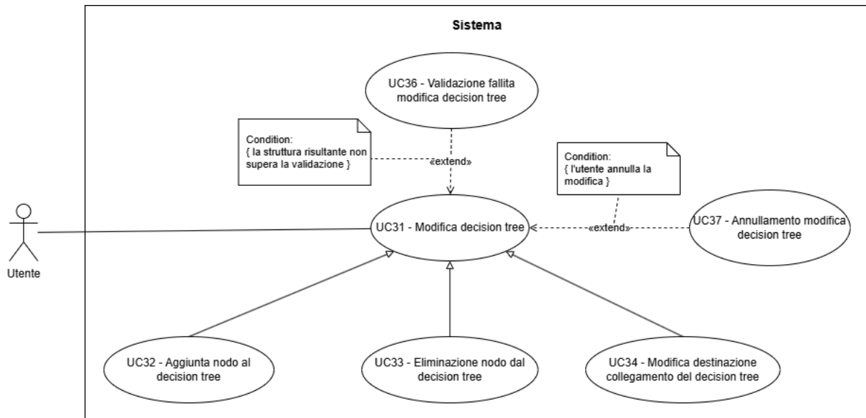
UC-31 : Modifica decision tree G
