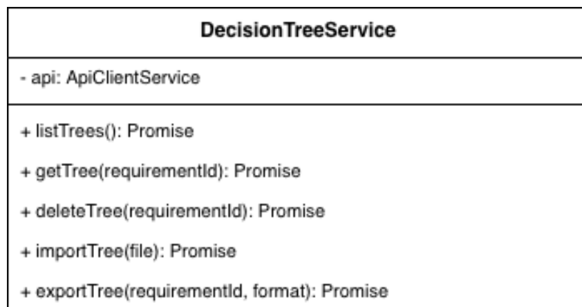
Figura 3: DecisionTreeService: classe application
