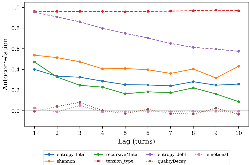
Turn-Level Autocorrelation by Lag
