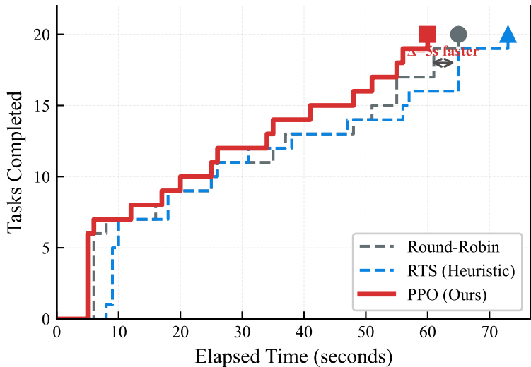
Cumulative Task Completion Over Time
