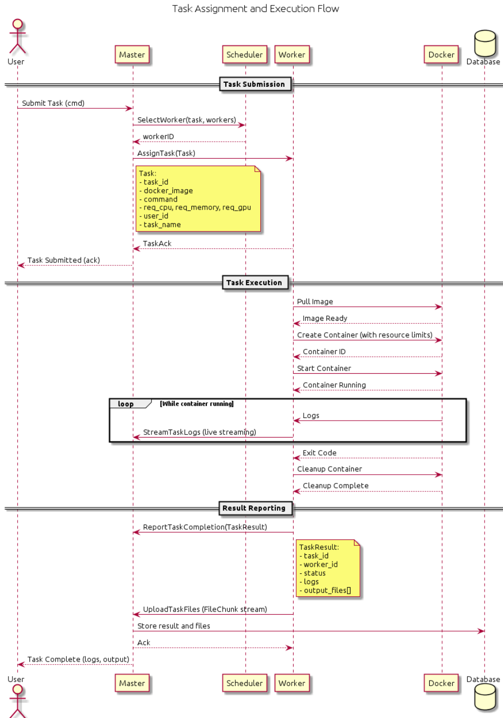
Figure 3.8.1: Task assignment and execution flow
