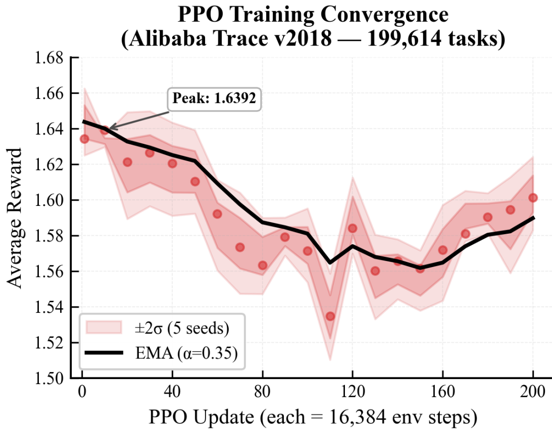
Figure 5.2.1: PPO training reward curve
