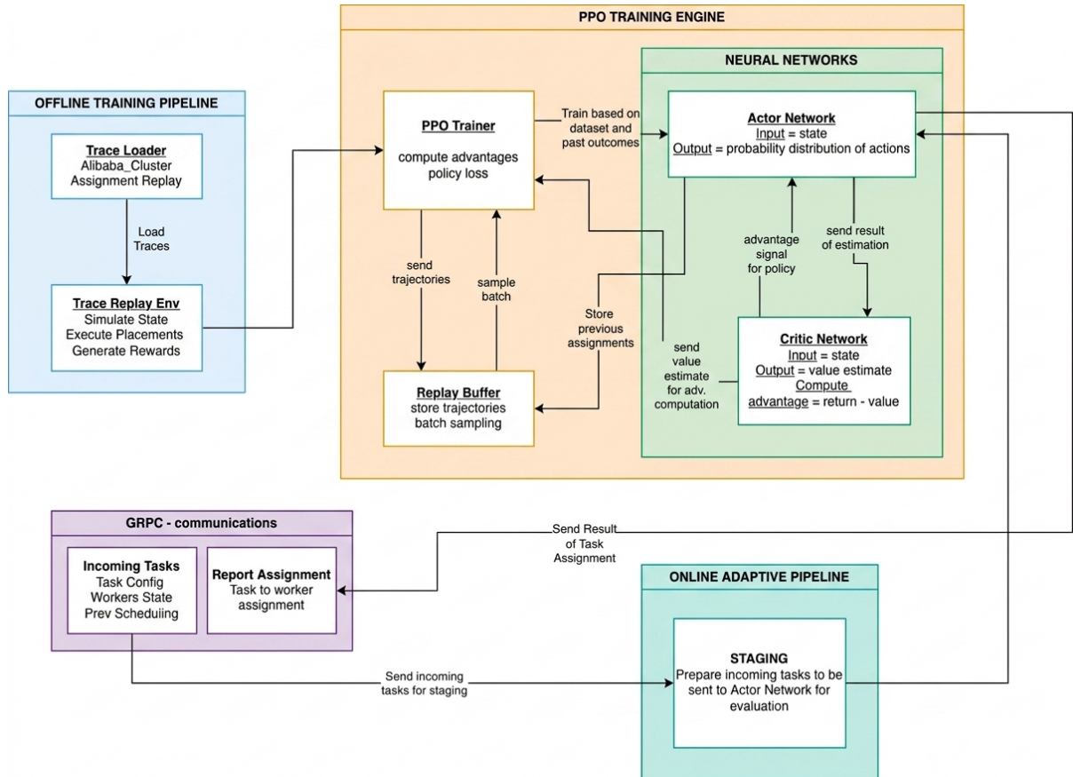
Figure 4.5.1: PPO scheduler architecture
