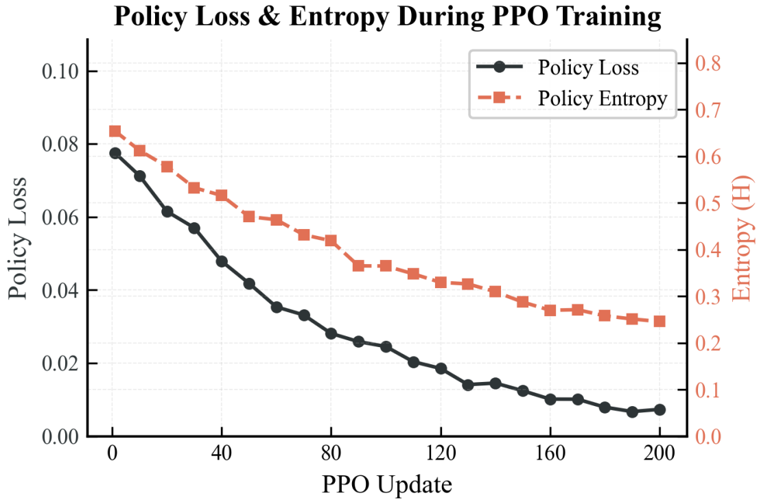
Figure 5.2.2: PPO policy loss and entropy
