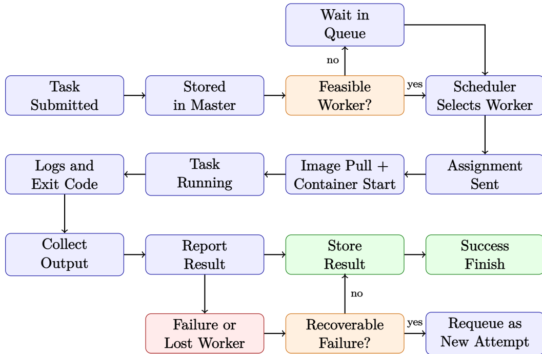
Figure 3.7.1: Task lifecycle in the cluster
