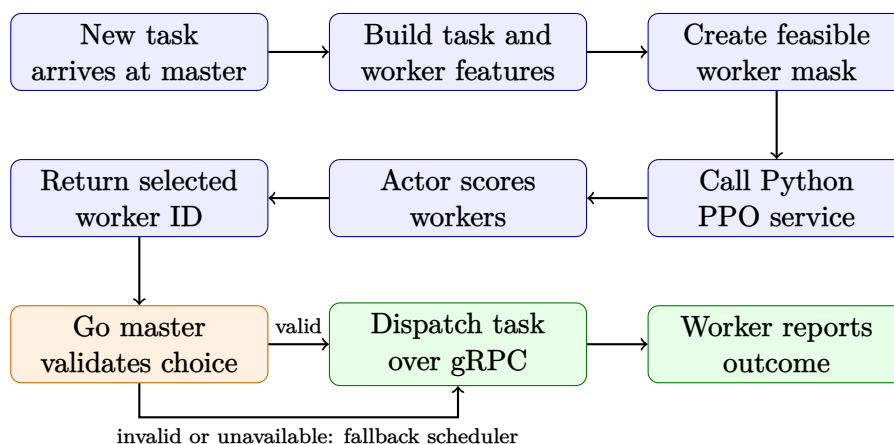
Figure 4.12.1: PPO scheduling flow inside the Go cluster
