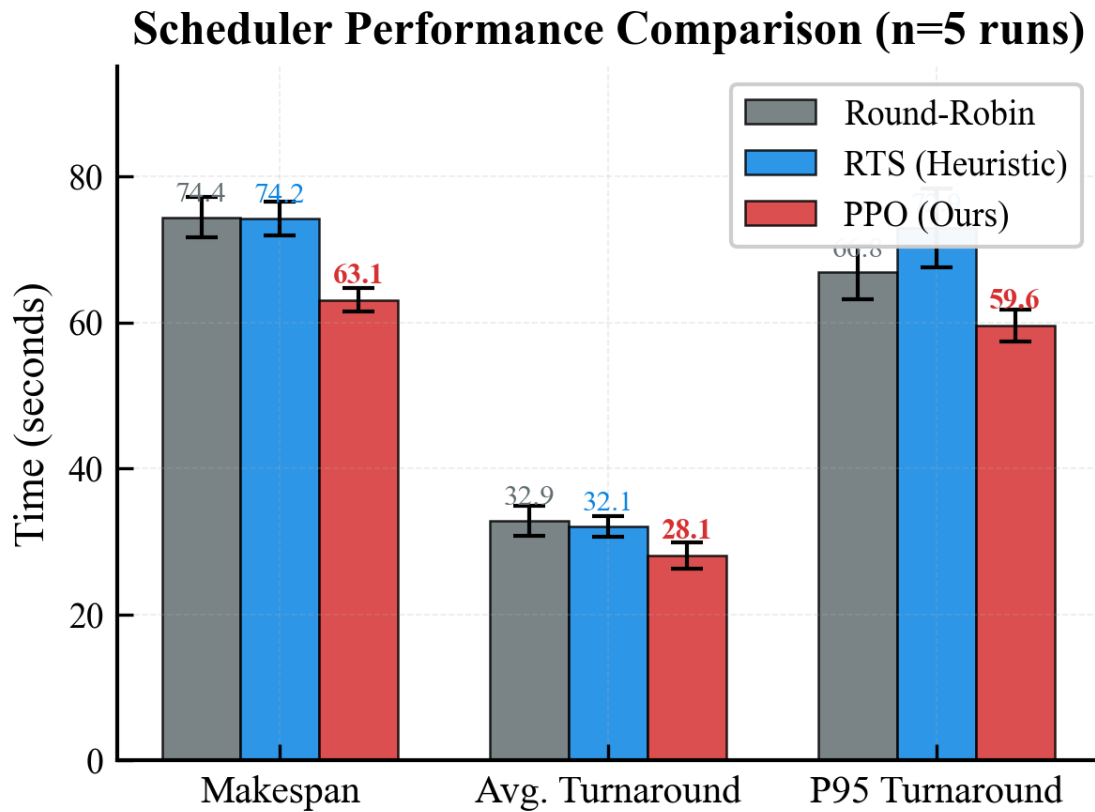
Figure 5.4.1: KPI comparison between schedulers
