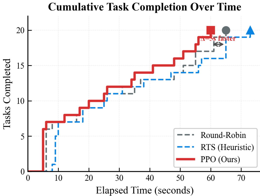
Figure 5.6.1: Cumulative task completion over time
