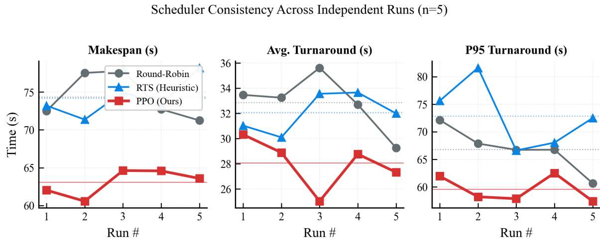
Figure 5.5.1: Multi-run scheduler comparison
