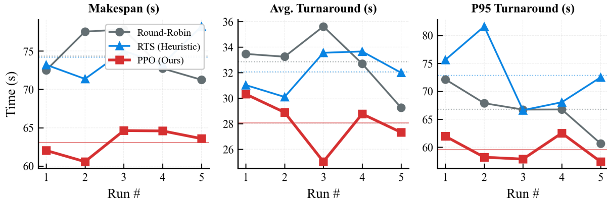
Figure 4.1.4: Multi-run scheduler comparison
