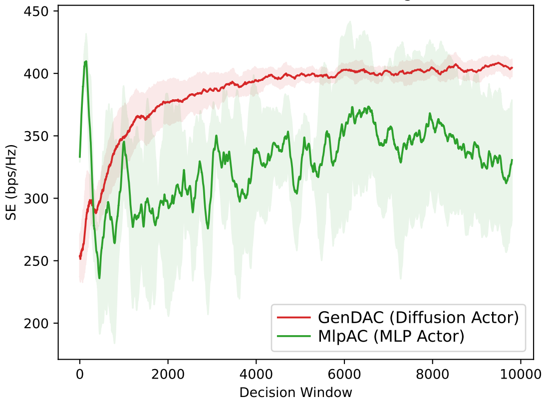
SE under Different Actor Design
