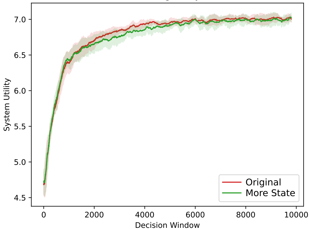
Training Utility
