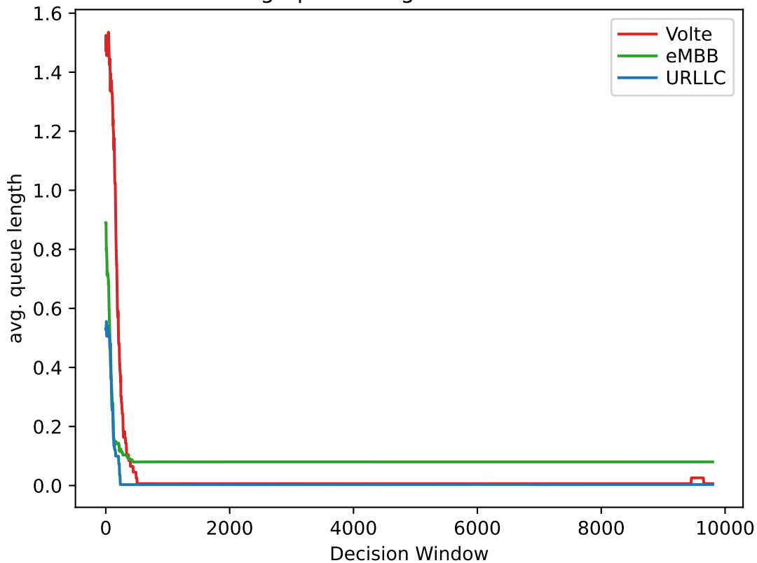
avg. queue length of each slice
