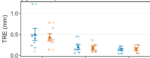
(a) CTChest, TRE
