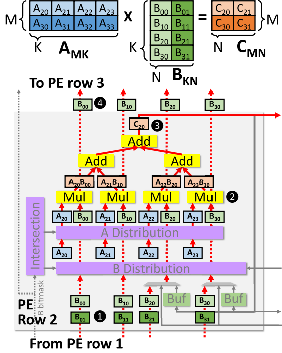
Fig. 7: Example of Trapezoid running IP for D \times D .
