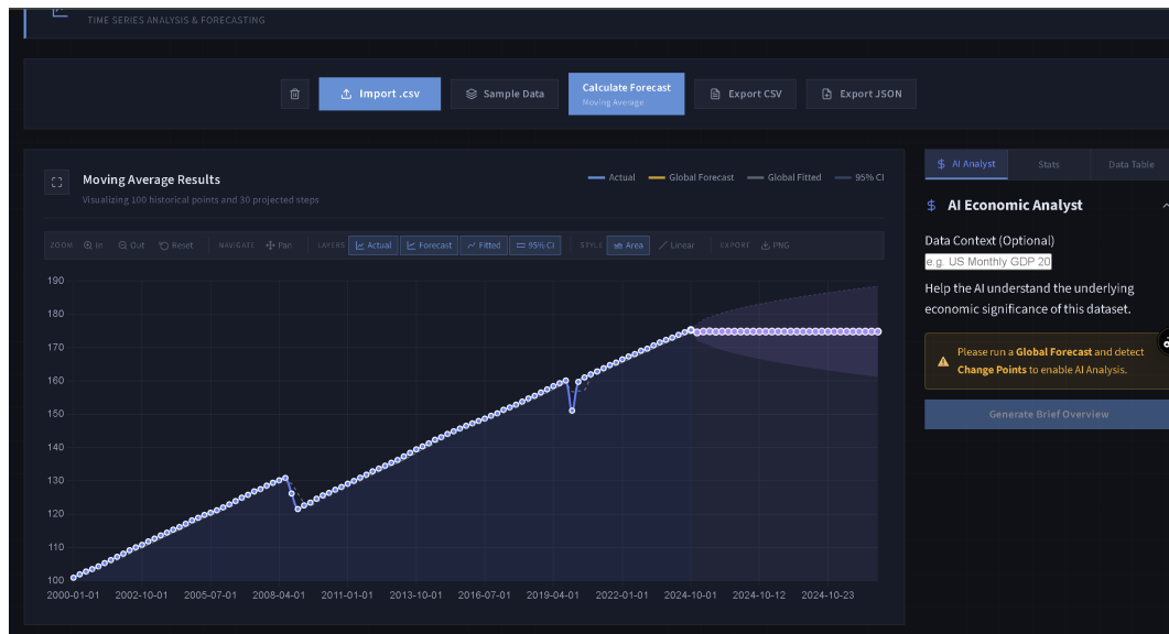
Figure 4.4: The HTML5 Canvas chart displaying a global Moving Average forecast alongside historical actual data and its corresponding 95% confidence interval bands.
