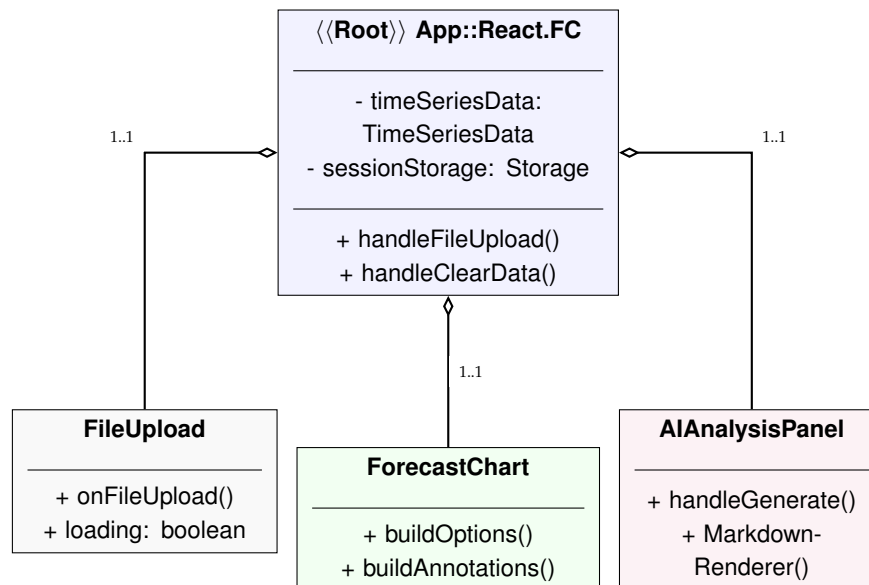
Figure 4.3: UML Class Diagram illustrating the React Structural Composition. The App root component securely aggregates all specialized sub-modules utilizing rigid, isolated TypeScript interfaces to prevent variable contamination.
