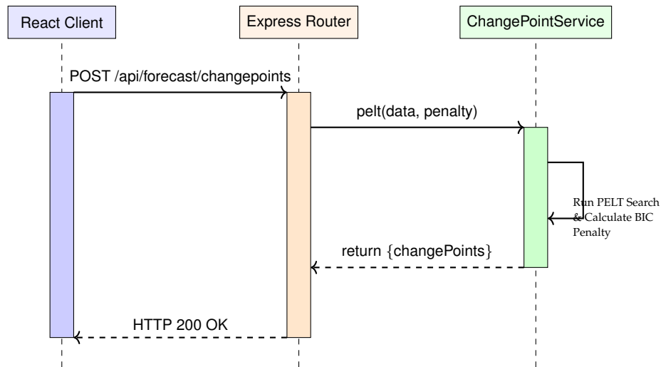
Figure 4.7: UML Sequence Diagram demonstrating the strict request lifecycle. The Express API handles the HTTP handshake, executing the PELT algorithm via the imported Service Module, before returning the boundaries and concluding the packet.
