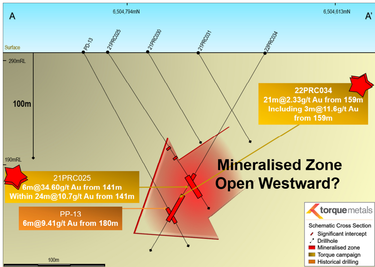
Figure 2: Paris Project 22PRC034 cross-section
