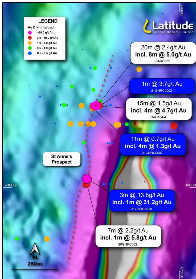
Figure 6: Plan showing St Anne's prospect, Au drilling intercepts overlaid on aeromagnetic image.
