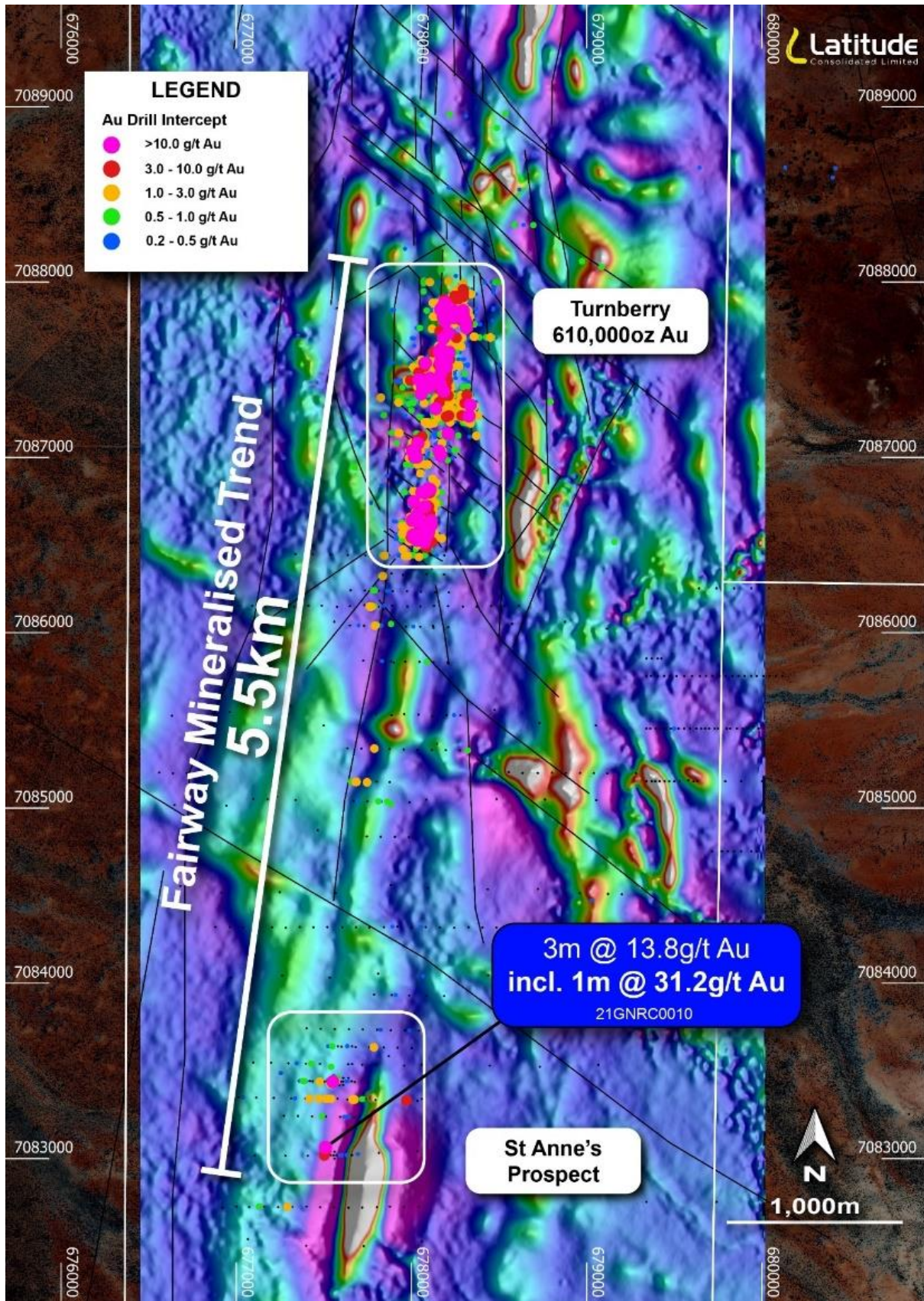
Figure 5: Plan showing the Fairway mineralised trend that extends from the Turnberry Mineral Resource to the St Anne's Prospect, Au drilling intercepts overlaid on aeromagnetic image.
