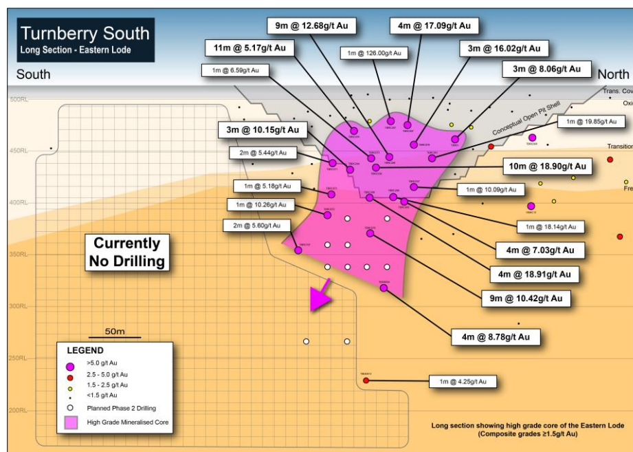
Figure 4: Section showing the Turnberry South high-grade shoot and Phase 2 drilling pierce points.
