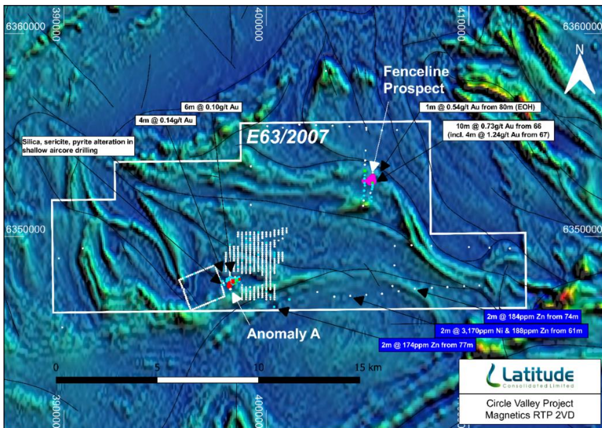
Figure 8: Circle Valley Gold Project aeromagnetic and drill results.
