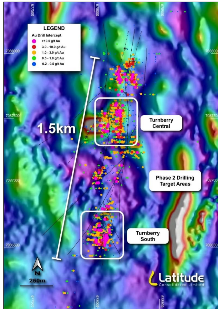
Figure 3: Plan showing the Turnberry Project, initial Phase 2 drilling targets and Au drilling intercepts overlaid on aeromagnetics.
