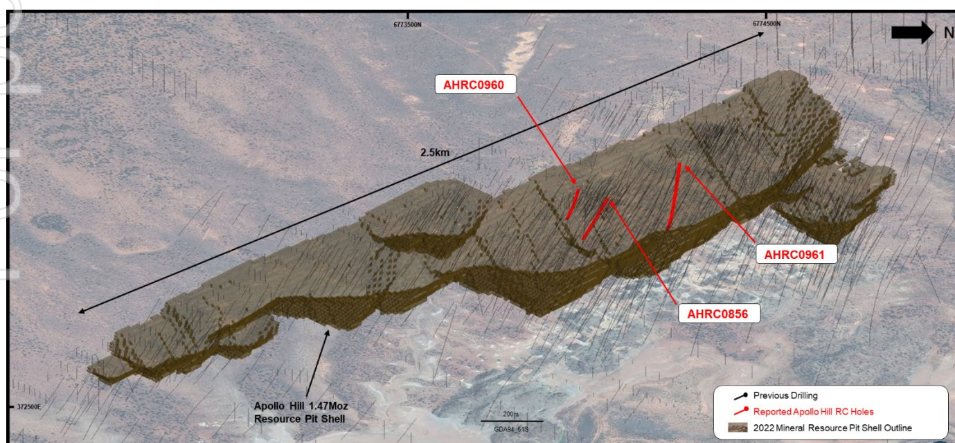
Figure 2 – Oblique view of the Resource Pit Shell, historical and reported drillhole traces.
