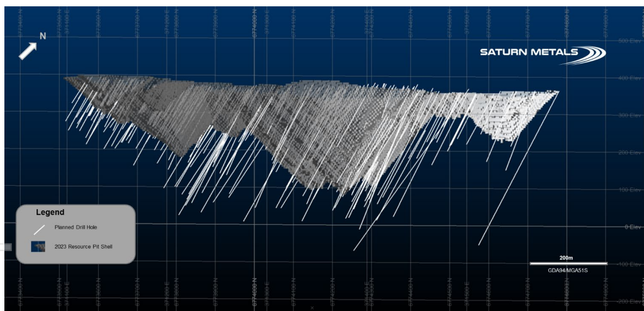
Figure 1 – Oblique View Looking Northwest of the Apollo Hill Resource Pit Shell (grey) with planned drilling (as white hole traces); demonstrating the extensional approach to the program.
