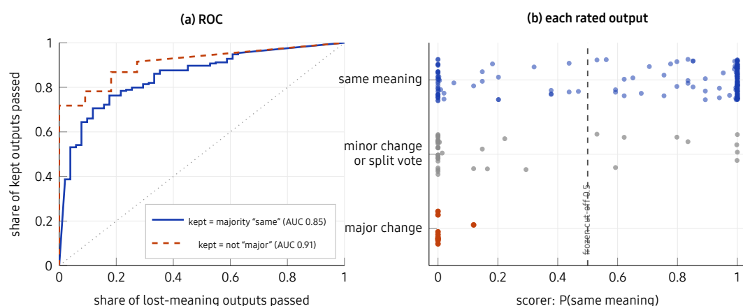
Figure 9. The meaning scorer against the raters, on 245 rated dev outputs. (a) ROC curves for two definitions of a kept meaning; the dotted diagonal is chance. (b) Every rated output by the raters’ majority answer (194 same, 40 minor or split, 11 major) against the scorer’s P(same); rows are jittered vertically for legibility.
