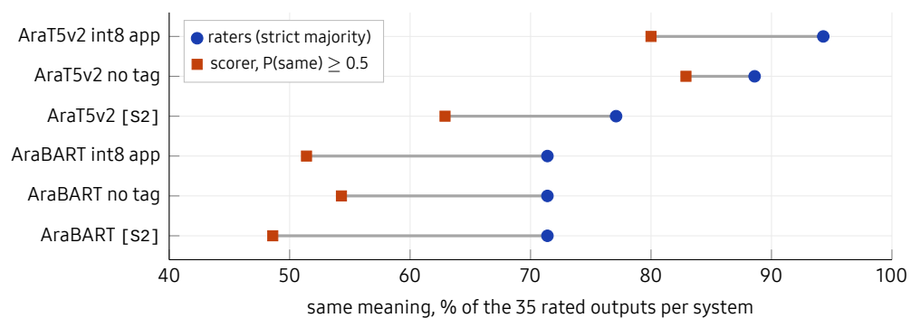
Figure 10. Same meaning, per system, on the same 35 outputs each: the raters' verdict (circle) and the scorer at P(\text{same}) \geq 0.5 (square).
