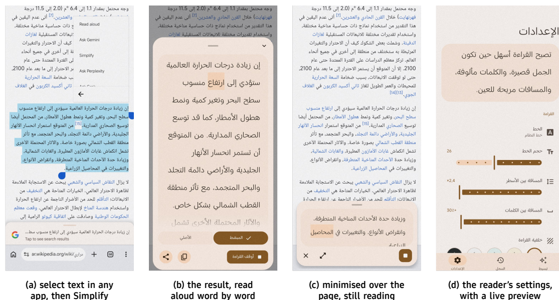
Figure 12. The app on the phone (Xiaomi Mi 11X), over an Arabic Wikipedia page, with the AraT5v2 bundle and a reader's own size and spacing; the phone's palette is seeded with the ochre of Bayan's logo. (a) The selection menu. (b) The result sheet, reading aloud with the current word highlighted. (c) Minimised over the page while reading continues. (d) Reading settings.
