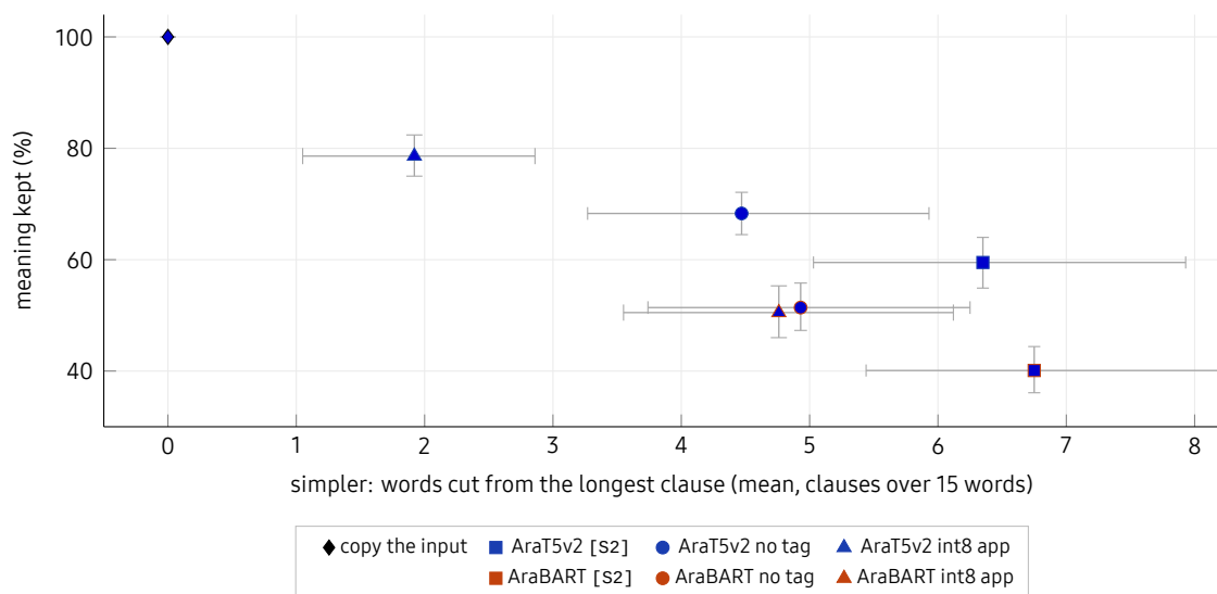
Figure 9. Meaning kept against simplification, test split, core items, with 95% document-bootstrap intervals. Copying the input sits at the top left by definition. Colour: the model; shape: the setting.
