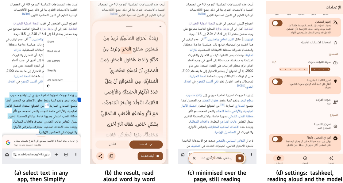
Figure 10. Bayan 2.1.0 on the phone (Xiaomi Mi 11X), over an Arabic Wikipedia page, with BayanSimplify-v0.3 (the large model, four beams), tashkeel shown and a reader's own size and spacing; the phone's palette is seeded with the ochre of Bayan's logo. (a) The selection menu. (b) The result sheet, reading aloud with the current word highlighted. (c) Minimised over the page while reading continues. (d) Settings: Show tashkeel , reading aloud, and the model with More faithful, slower .
