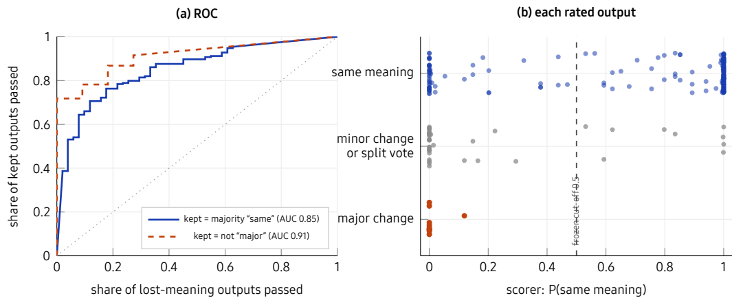
Figure 8. The meaning scorer against the raters, on 245 rated dev outputs. (a) ROC curves for two definitions of a kept meaning; the dotted diagonal is chance. (b) Every rated output by the raters' majority answer (194 same, 40 minor or split, 11 major) against the scorer's P(same); rows are jittered vertically for legibility.
