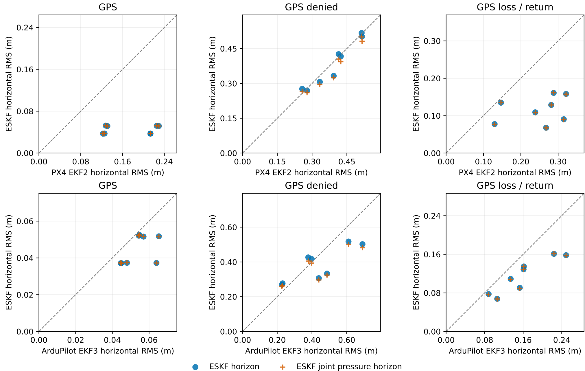
Eight matched captures per panel; points below the diagonal favor ESKF
