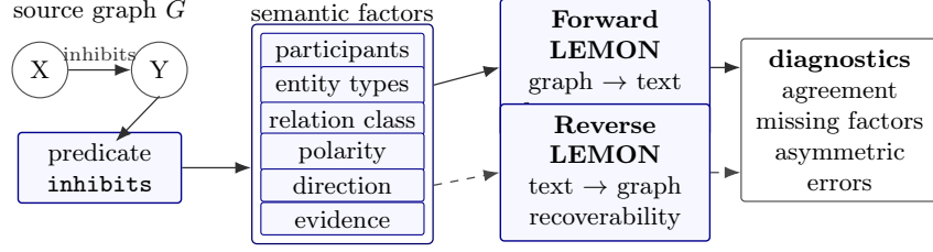
Fig. 1. Predicate-factor evaluation for graph-text alignment. A source predicate is decomposed into semantic factors, which are checked as forward graph-to-text coverage and reverse text-to-graph recoverability. Solid arrows denote forward evidence checks; dashed arrows denote reverse recovery checks.
