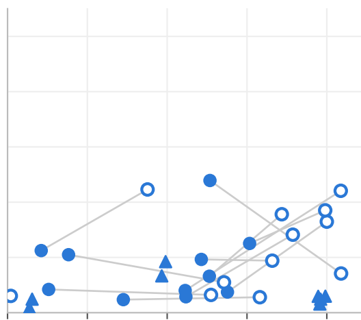
ExtraTrees
