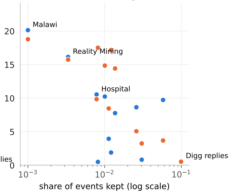
B · share of events kept
