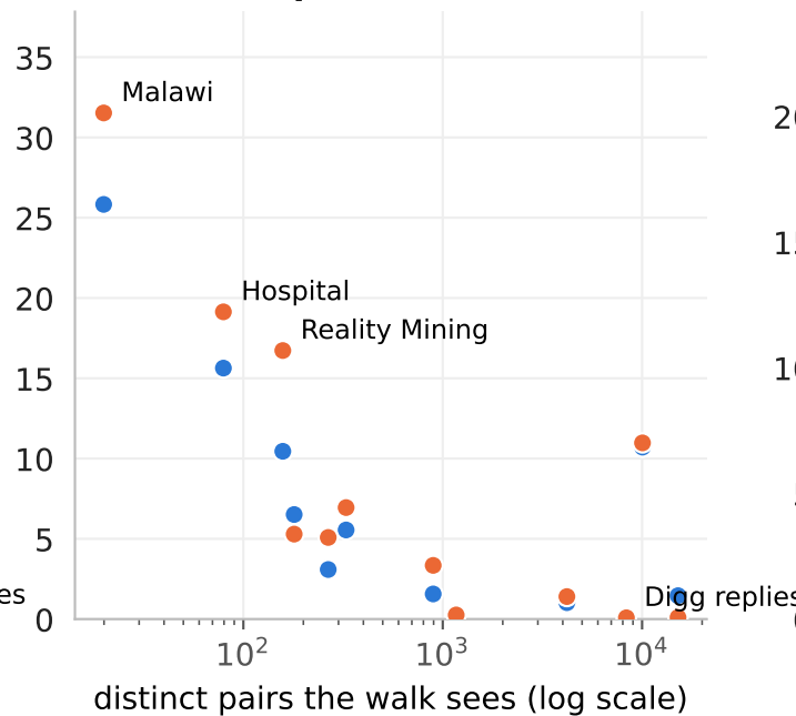
S · distinct pairs in the walk
