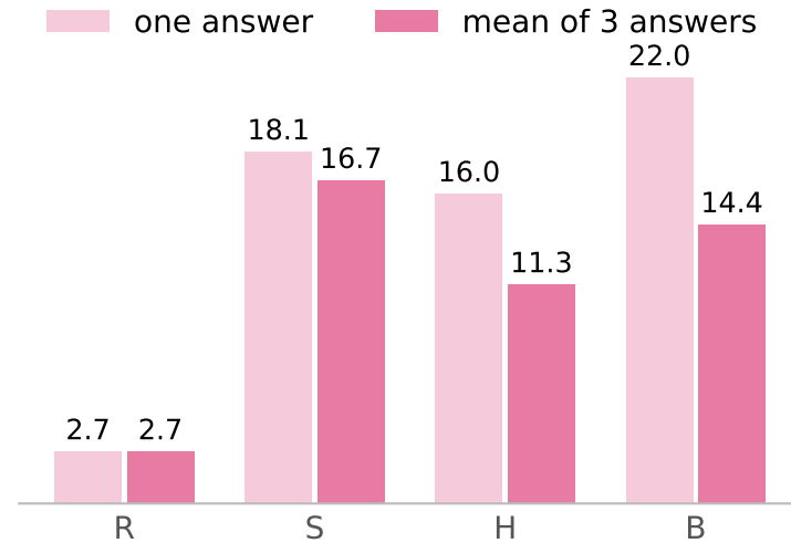
Qwen thinking: error (pp)
