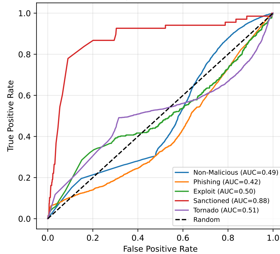
Logistic Regression Recipient Address ROC
