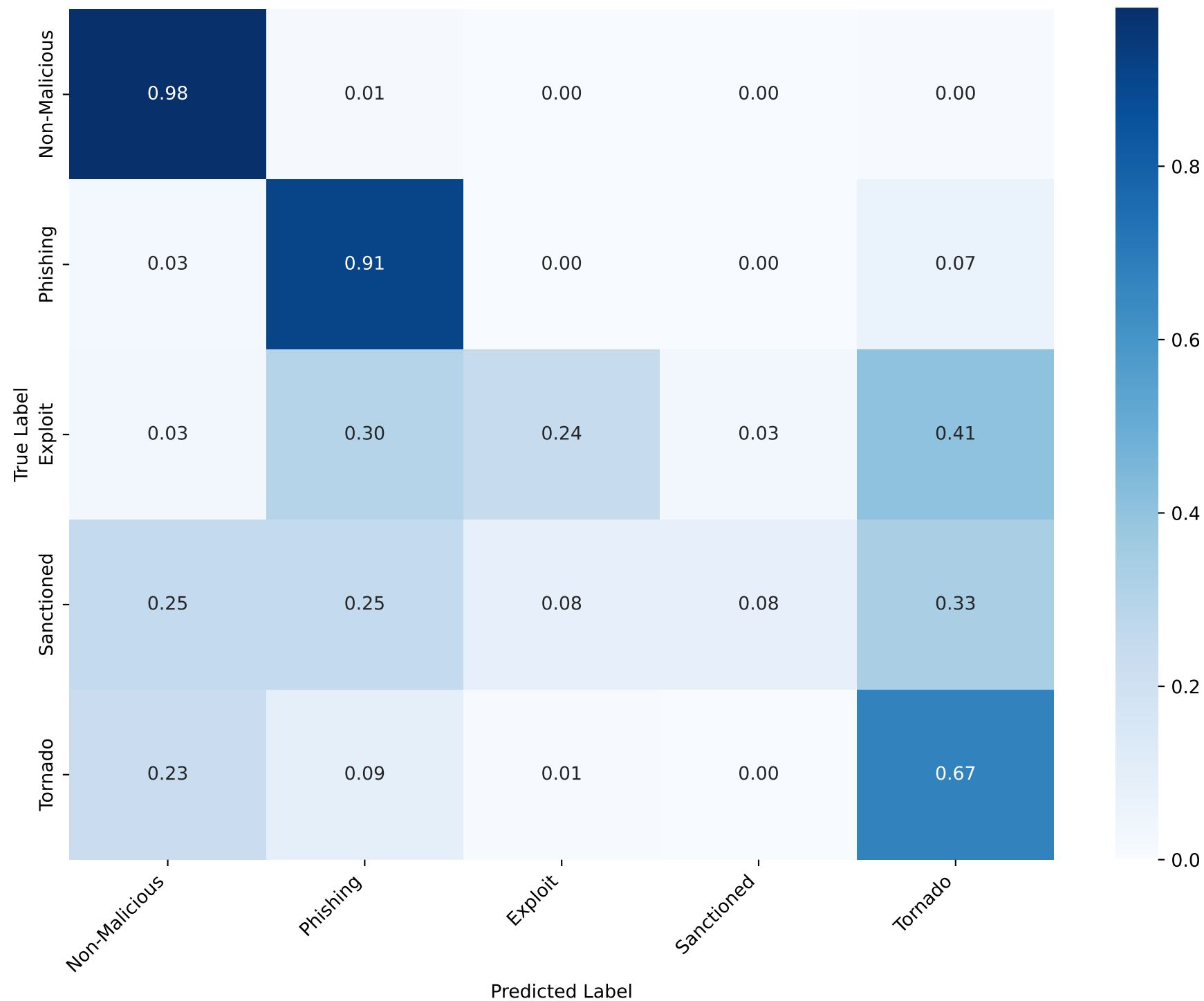
Model 1: Address Classification - RandomForest
