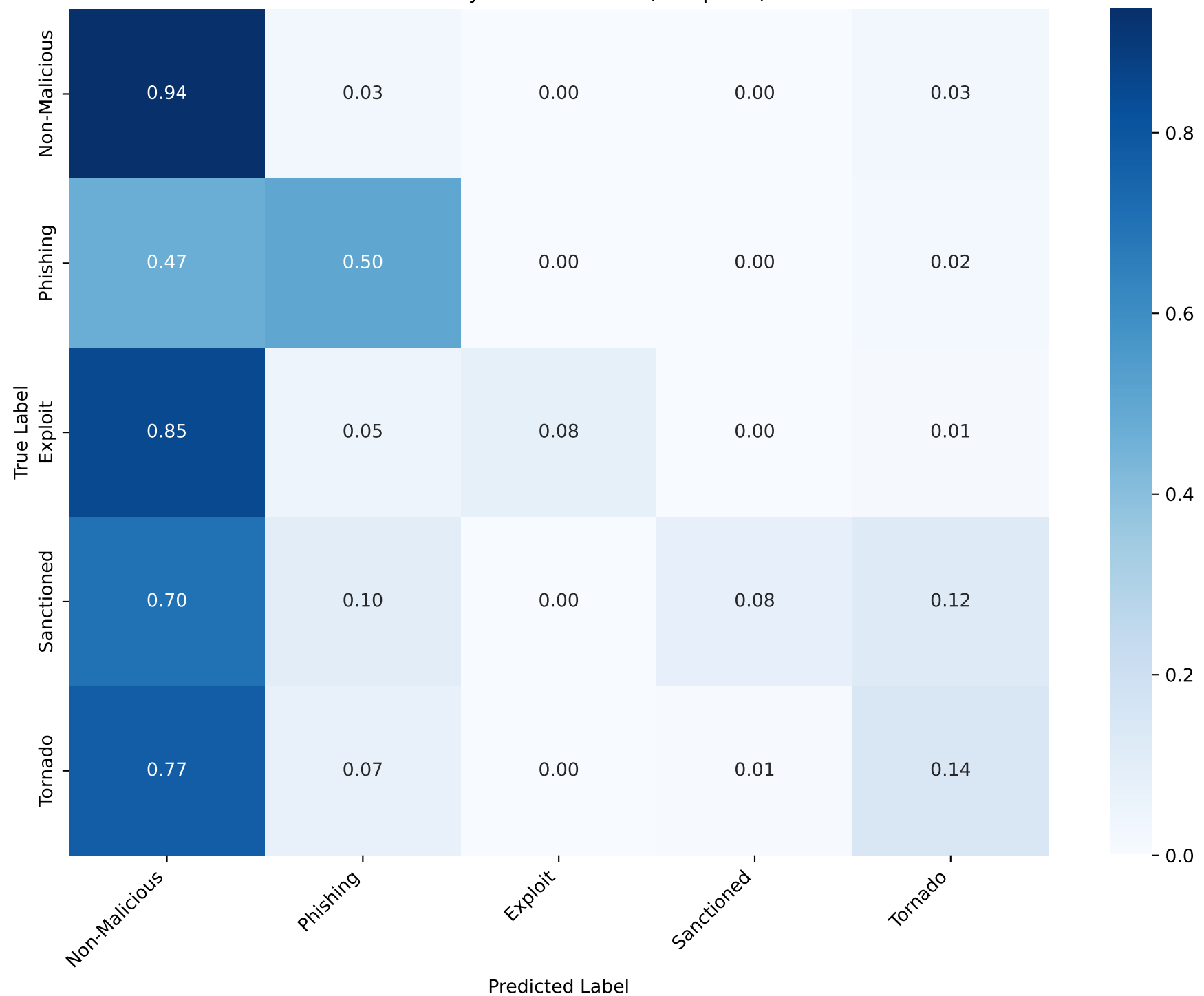
Model 3: Hybrid - XGBoost (Recipient)
