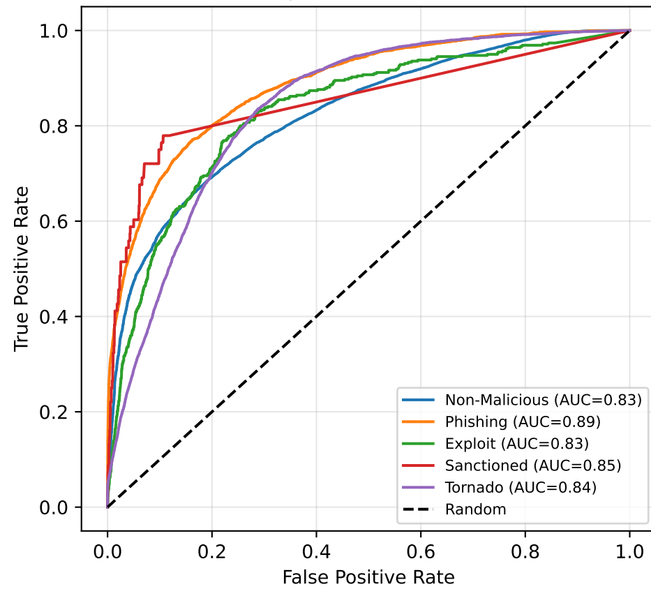
Random Forest Recipient Address ROC
