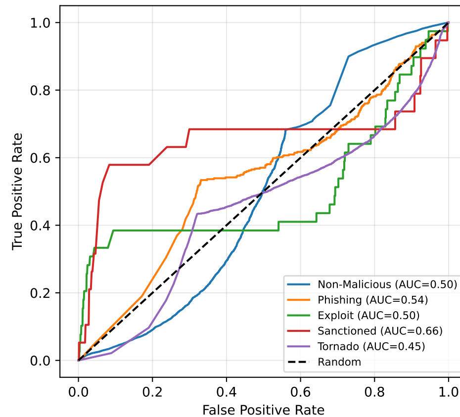
Logistic Regression Source Address ROC
