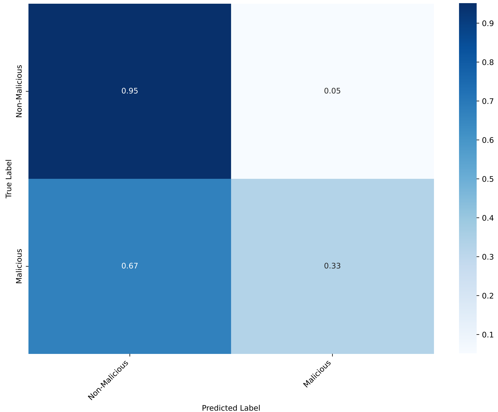
Model 2: Transaction Classification - XGBoost
