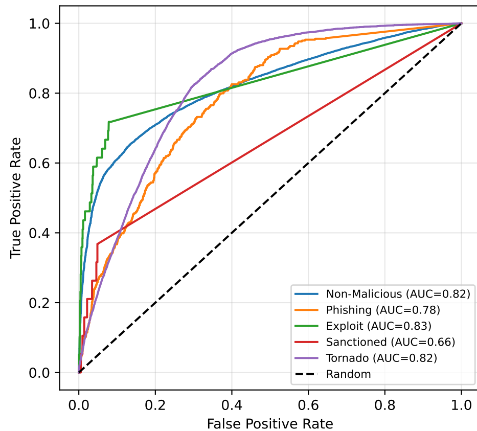
Random Forest Source Address ROC
