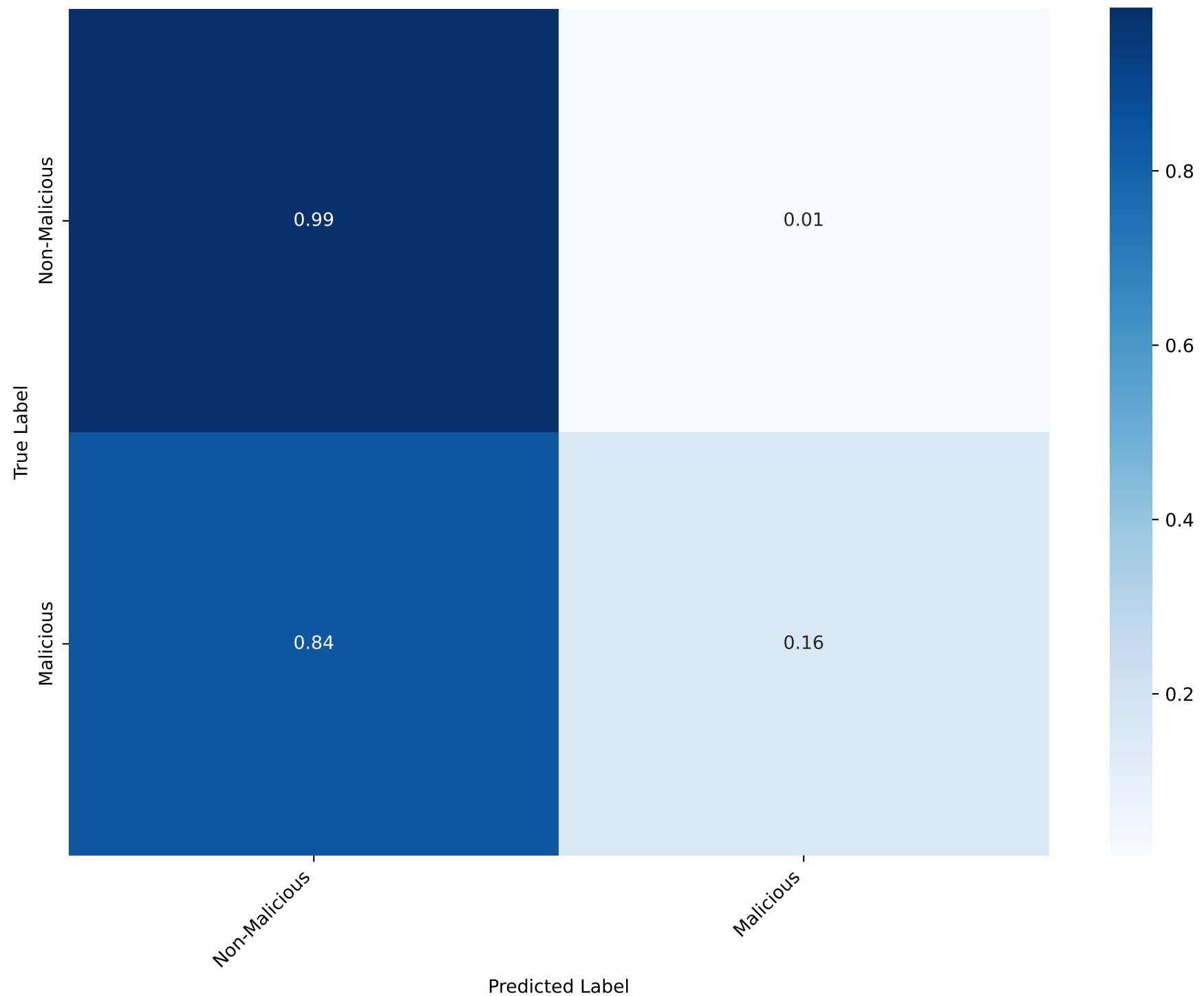
Model 2: Transaction Classification - RandomForest
