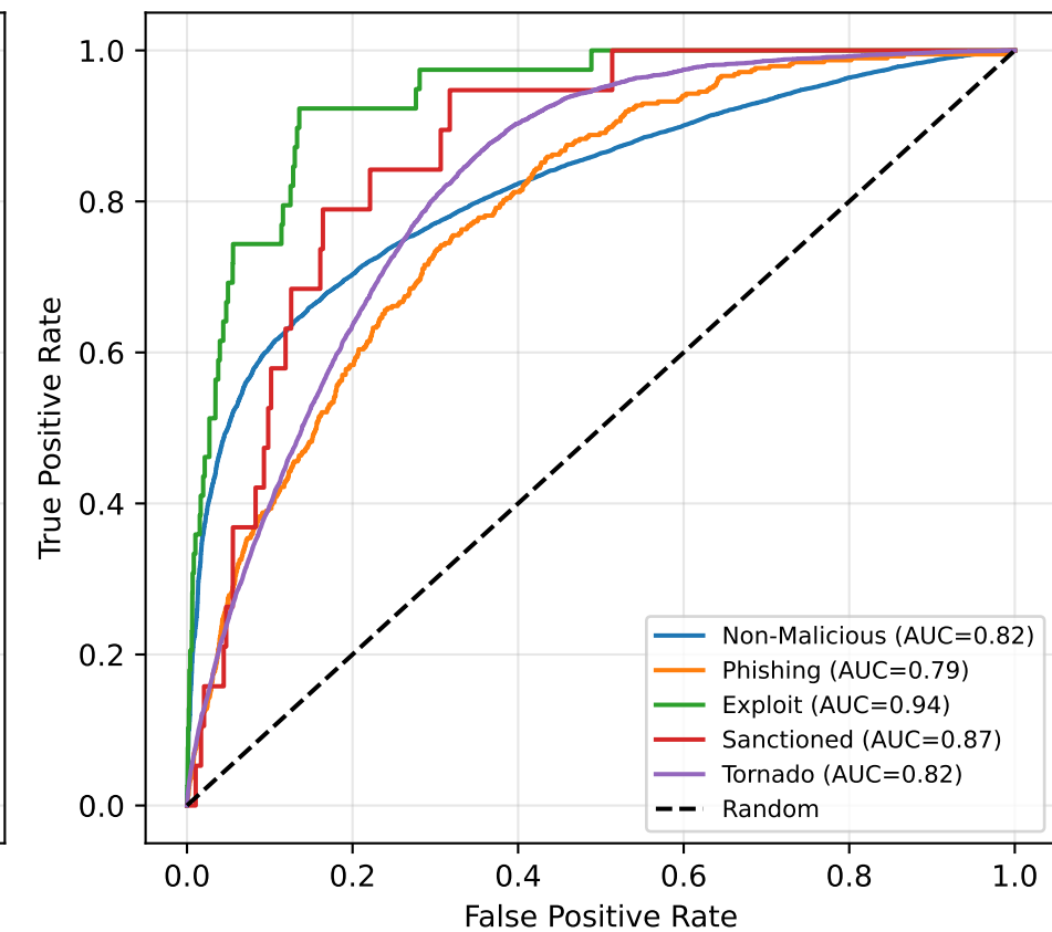
XGBoost Source Address ROC
