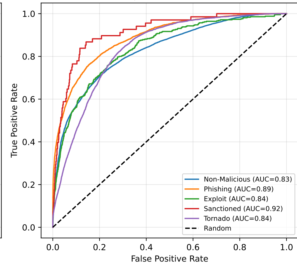
XGBoost Recipient Address ROC
