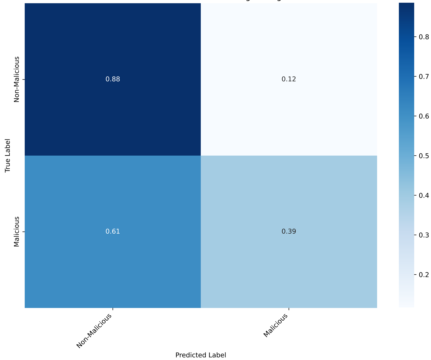
Model 2: Transaction Classification - LogisticRegression
