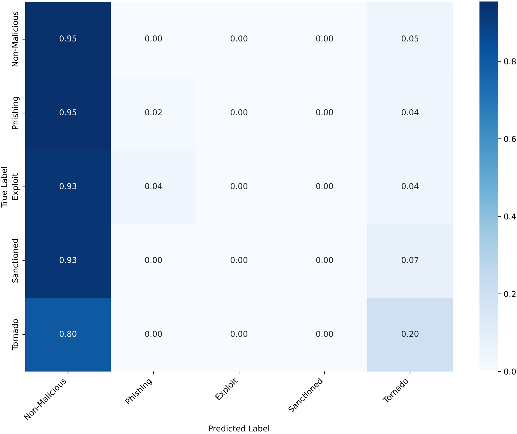
Model 3: Hybrid - RandomForest (Source)
