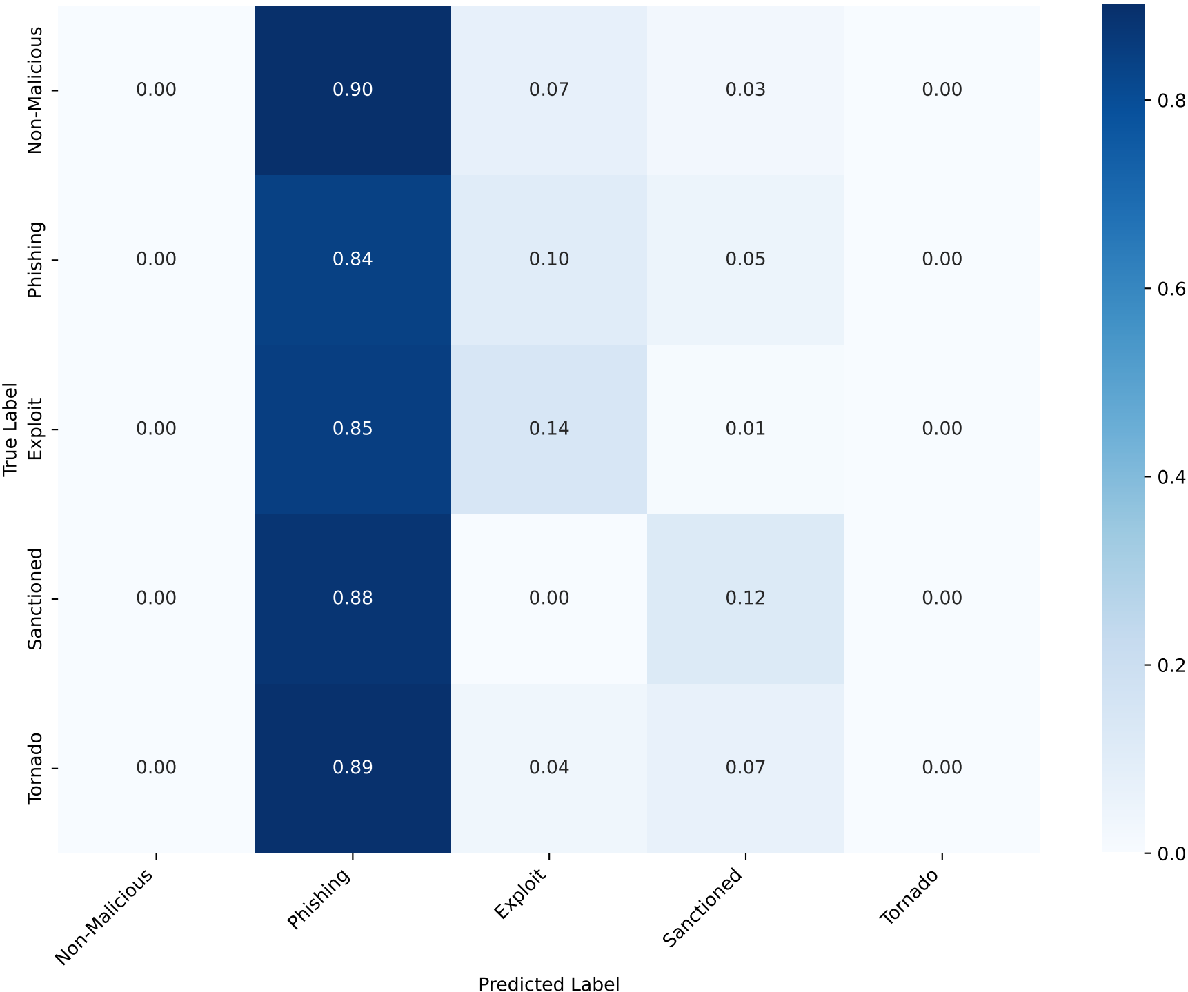
Model 3: Hybrid - LogisticRegression (Recipient)
