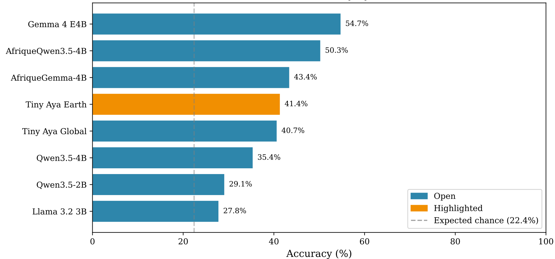
SUB: Overall Accuracy by Model
