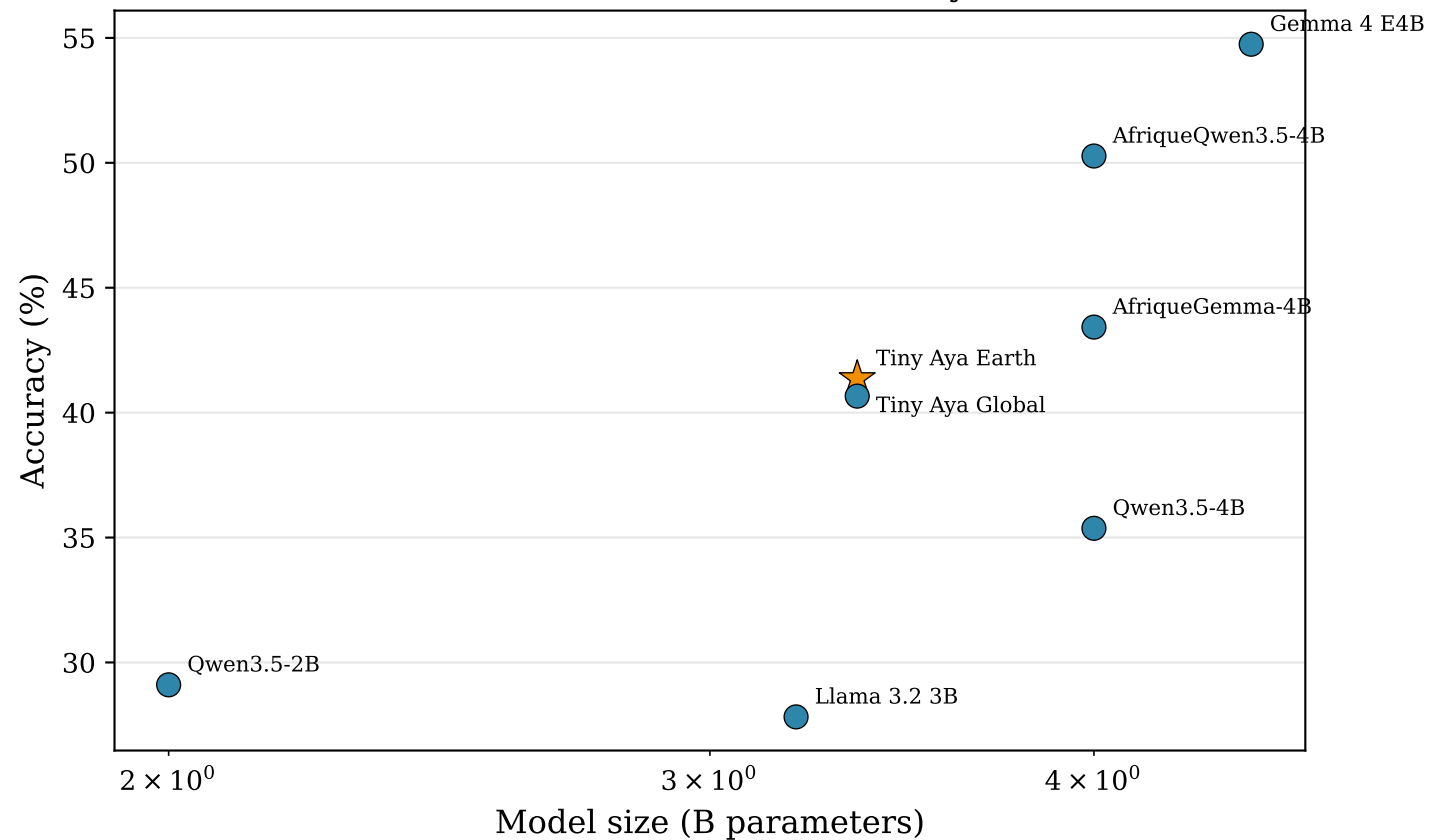
SUB: Model Size vs Accuracy
