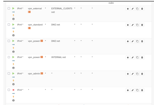
Figure 1. OpenVPN interface rules on the Main firewall.
