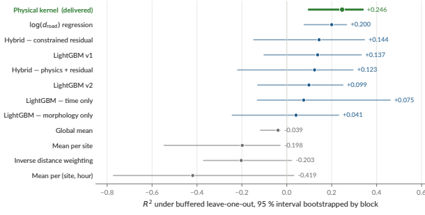
Figure 3: Every model under the reference protocol with its 95 % interval. The physical kernel is the only model whose interval excludes zero under all three protocols — and it is not separated from the two-parameter distance regression.
