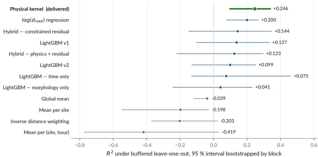
Figure 8: Every model under the reference protocol with its 95 % interval. The physical kernel is the only model whose interval excludes zero under all three protocols — and its interval overlaps that of the two-parameter distance regression almost entirely (§5.3).
