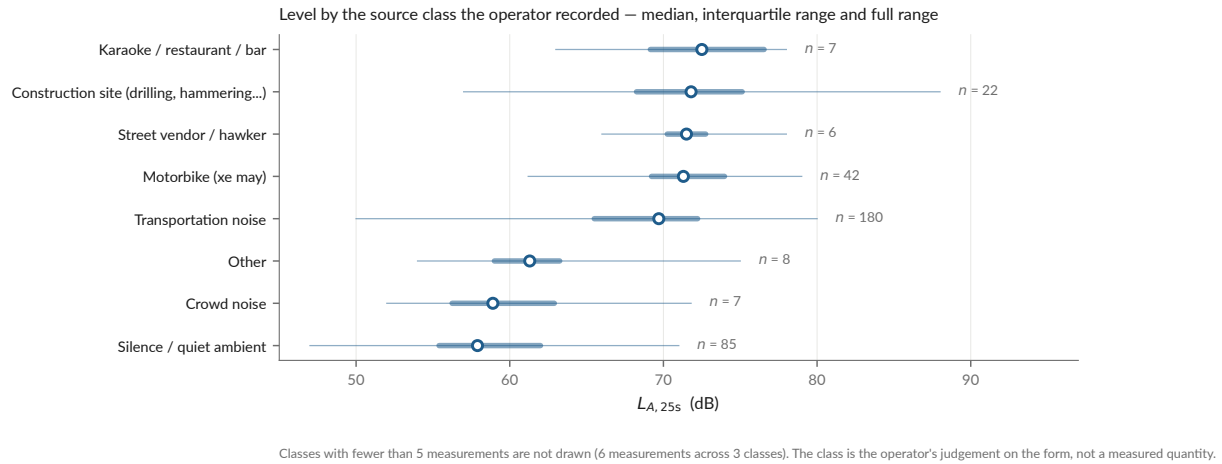
Figure 5: Level against the source class the operator selected on the form — the one variable in the dataset that is a human judgement rather than a sensor reading. It behaves: the ordering it produces is the ordering the physics predicts, karaoke and construction at the top, declared silence at the bottom, with no reordering needed. It also shows how unbalanced the campaign is — transportation noise and silence carry three quarters of it. Recomputed from data/processed/measurements.csv .
