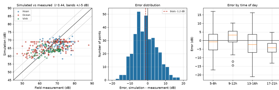
Figure 11: Simulated against measured levels, n = 360 matched points ( results/tables/validation_simulation.csv , scripts/08_validate_simulation.py ). Mean error -1.24 dB, MAE 5.30 dB, RMSE 6.49 dB. The simulation reproduces the spatial and temporal ordering; it does not reproduce the spread, which is expected given that features aggregated over 300 m cannot resolve the facade/courtyard contrast.
