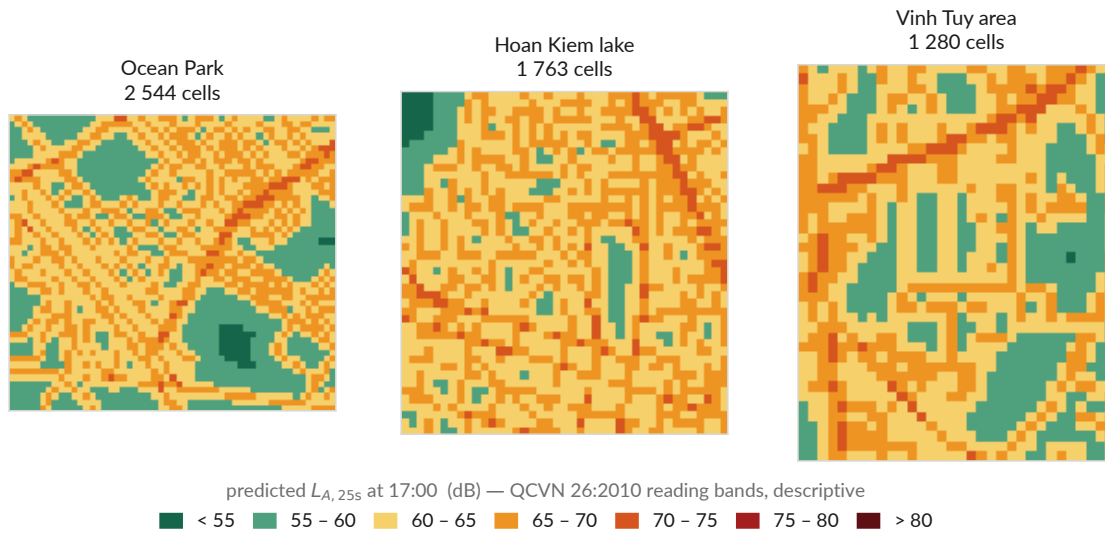
Figure 10: The published 40 m grid, redrawn from the CSV rather than screenshots. QCVN 26:2010 colour bands, used descriptively.
