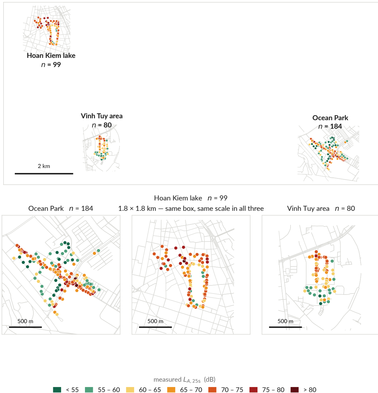
Figure 2: Where the 363 measurements actually are. Top: all three areas in one frame, on the street network each was measured in, coloured by the level measured there. Bottom: each area cut to the same 1.8×1.8 km box, so the three densities can be compared by eye — panels scaled to their own data would make the sparsest site look the busiest. The blank space in the top panel is the argument of this report in one picture: the campaign is three islands roughly 11 km apart, and the model of §4.5 is asked to generalise across everything between them, which was never measured. There is no basemap and no tile server here — roads are the OSMnx extracts the GAMA simulation already runs on ( simulation/gama/inputs/ ), so nothing on this figure comes from outside the repository. scripts/12_presentation_figures.py .
