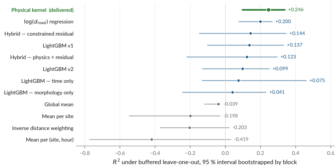
Figure 5: Every model under the reference protocol with its 95 % interval. The physical kernel is the only model whose interval excludes zero under all three protocols — and its interval overlaps that of the two-parameter distance regression almost entirely (§5.3).
