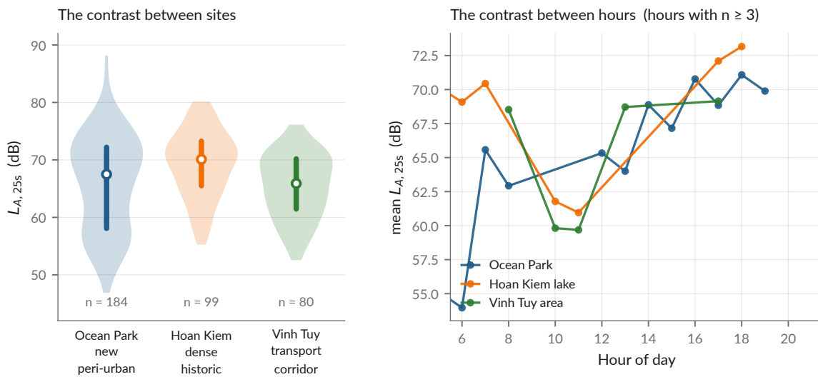
Figure 2: The 363 measurements: spatial layout, level distribution and temporal coverage. Produced by scripts/12_presentation_figures.py from data/processed/measurements.csv and models/metrics.json .
