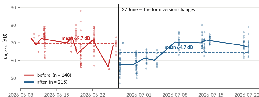
Figure 9: The level distribution around 27 June 2026. The break date is not chosen by the figure: it is the date the form version changes. Produced by scripts/12_presentation_figures.py from data/processed/measurements.csv .
