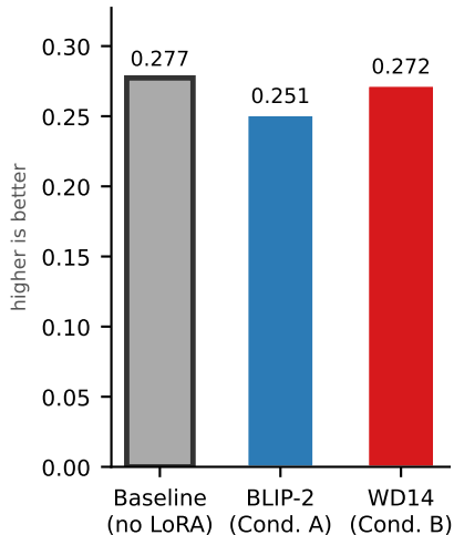
CLIP score
