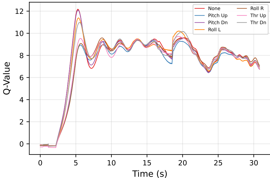
Q-Value Evolution
