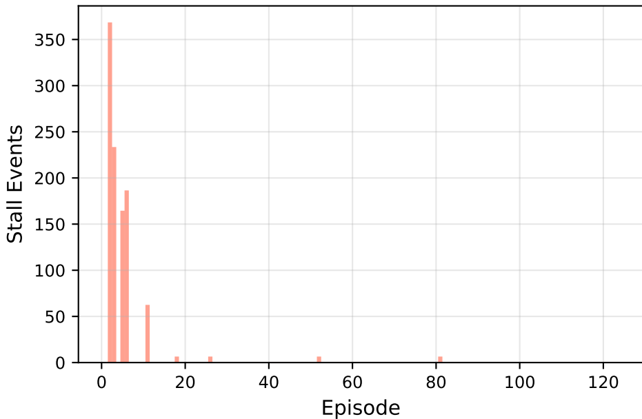
Stall Frequency Over Training
