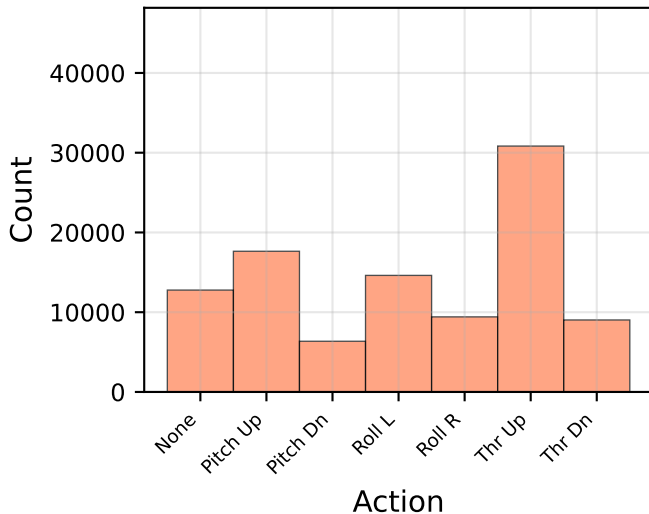
Early Training
