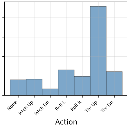
Late Training
