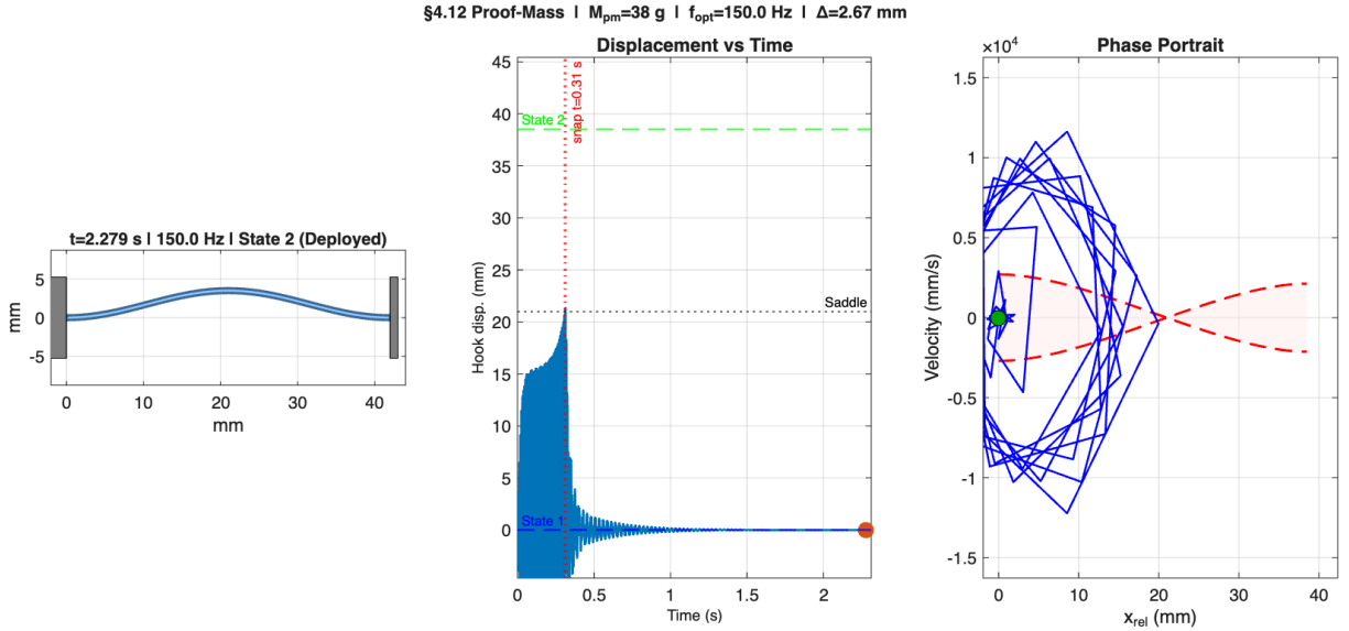
Figure 4: Animation snapshot for the proof-mass actuator at the optimal proof-mass parameter. The proof mass oscillates on the motor output shaft, driving the plate and hook into snap-through.
