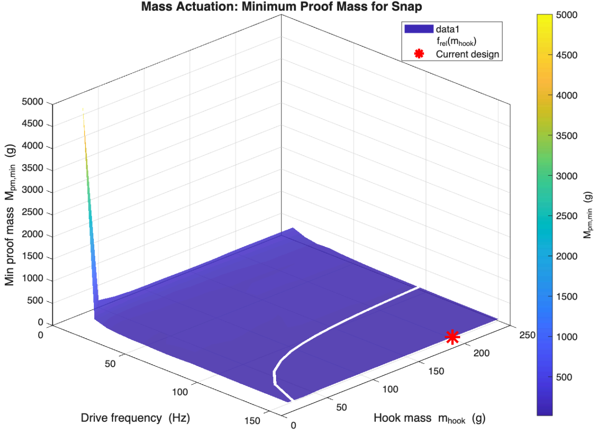
Figure 5: M_{\text{pm,min}} vs. drive frequency and hook mass m_h .
