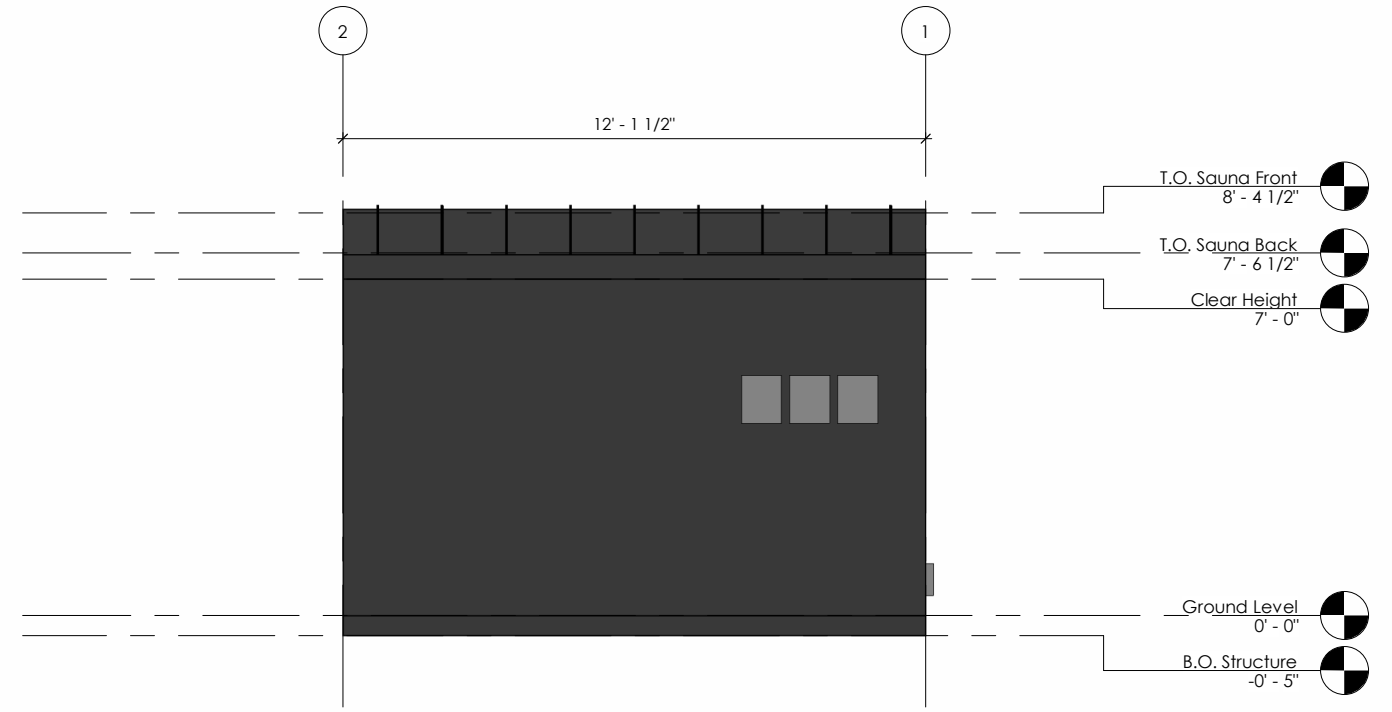
② Back 1/4" = 1'-0"
