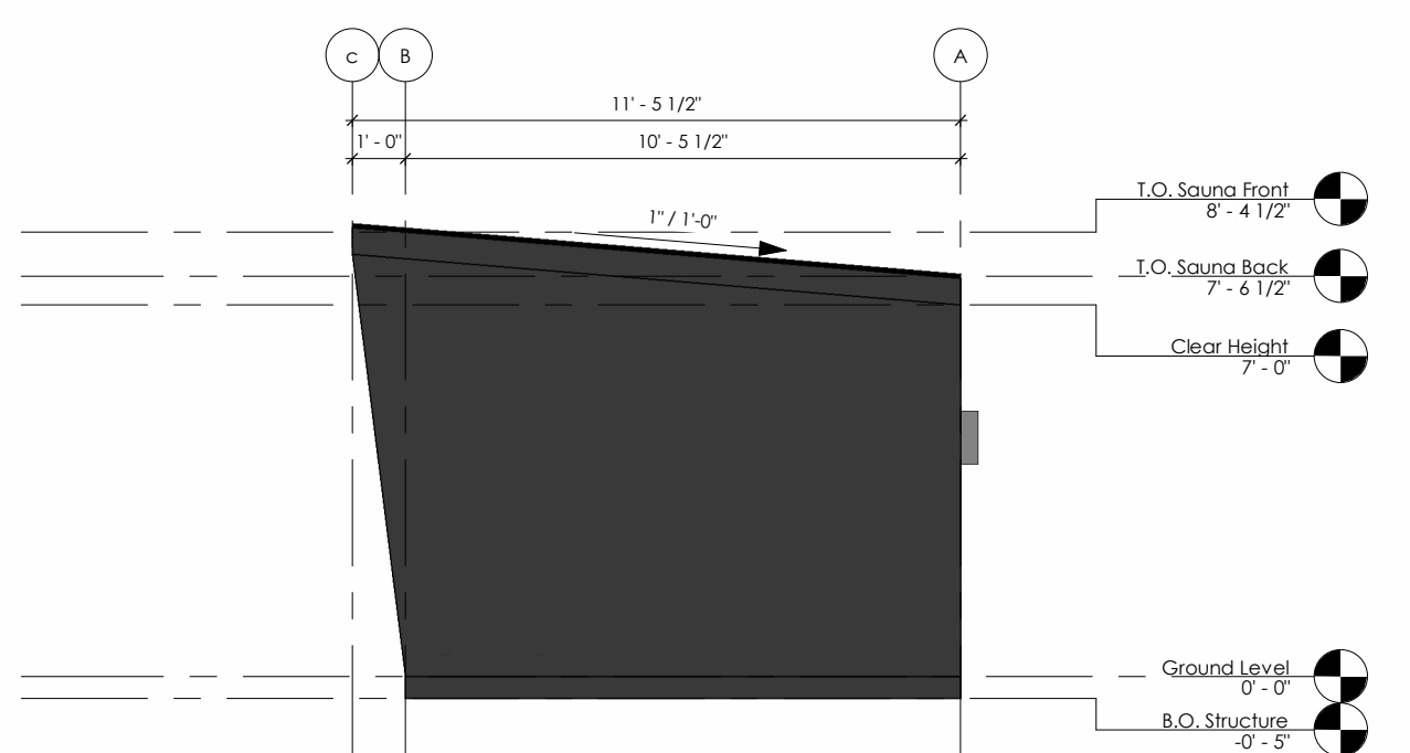
④ Right 1/4" = 1'-0"
