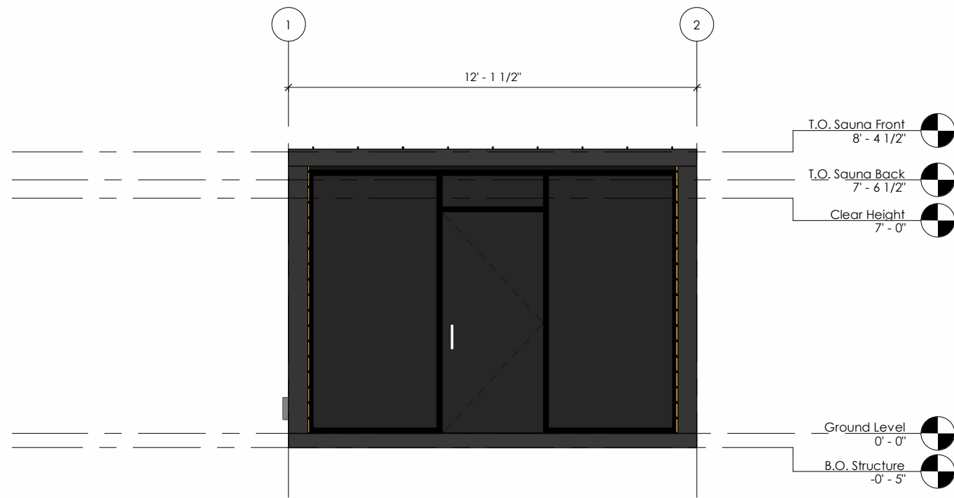
① Front 1/4" = 1'-0"
