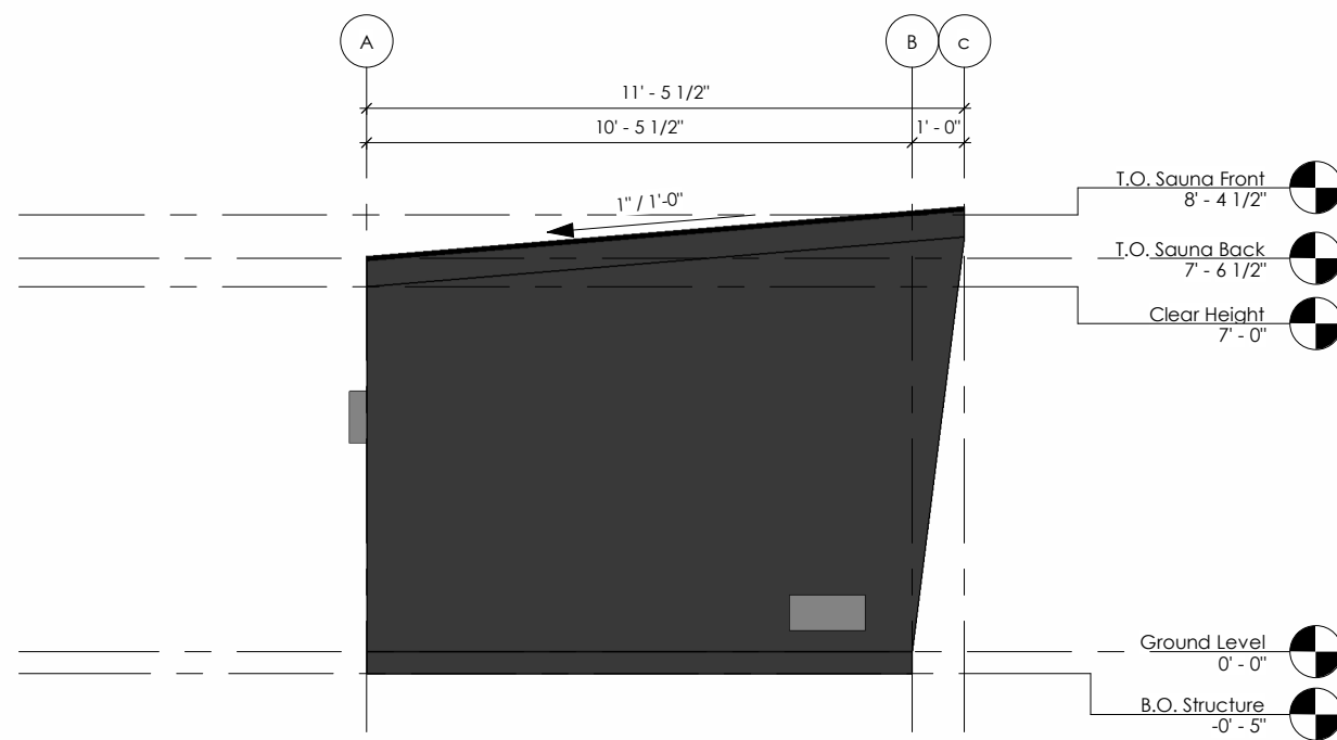
③ Left 1/4" = 1'-0"
