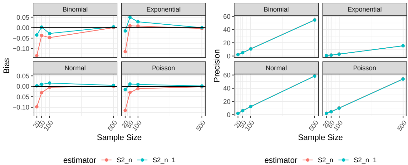
Figure 2: Sample Size vs Bias and Precision
