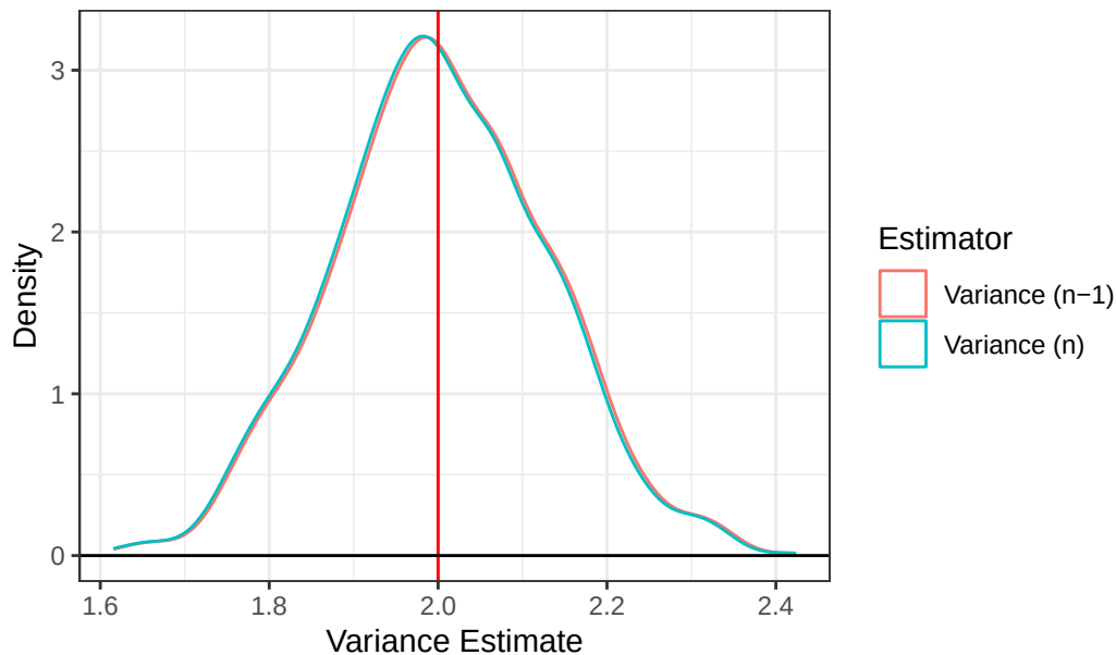
Normal, n = 500
