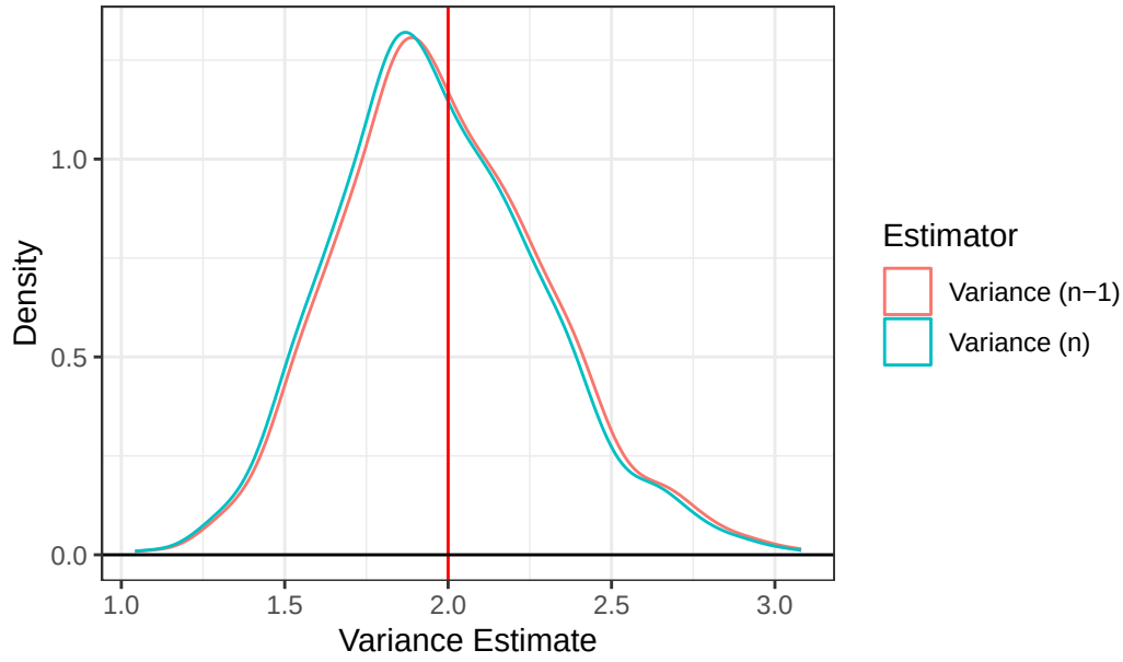
Binomial, n = 100
