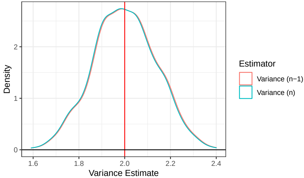
Binomial, n = 500
