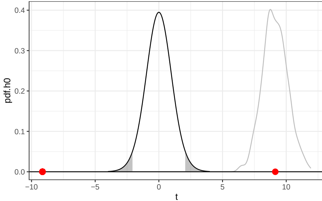
Figure 4: T distribution with rejection region shown
