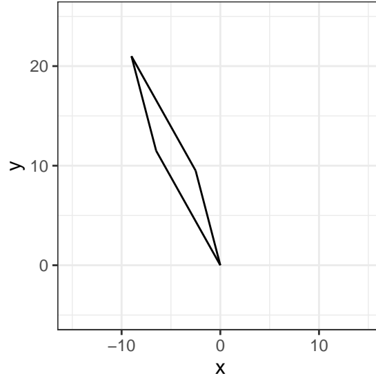
Figure 6: The shape for T = A * Mvh .
