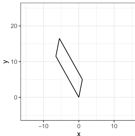
Figure 4: The shape for T = A \cdot M_v .
