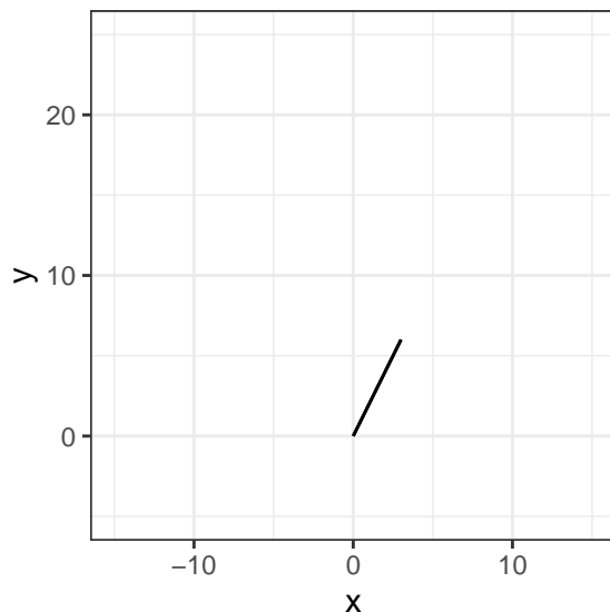
Figure 3: The shape for T = AM .
