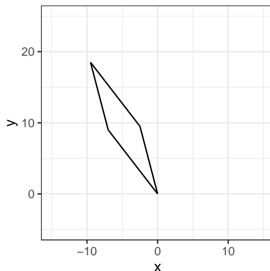
Figure 5: The shape for T = A * M_h .
