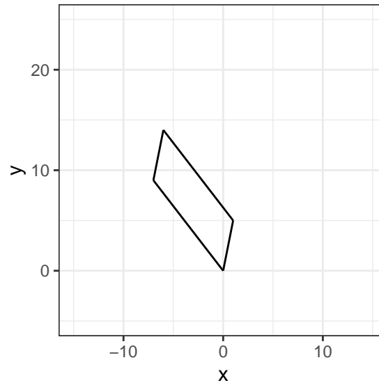
Figure 2: The shape for T = AM .
