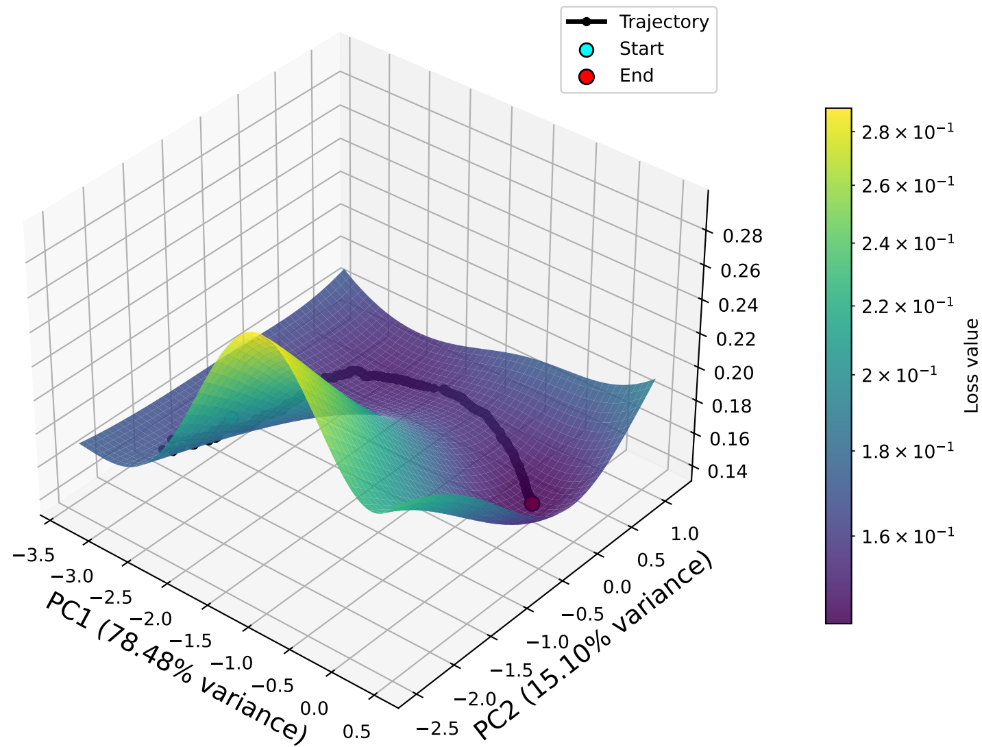
PCA Loss Landscape
