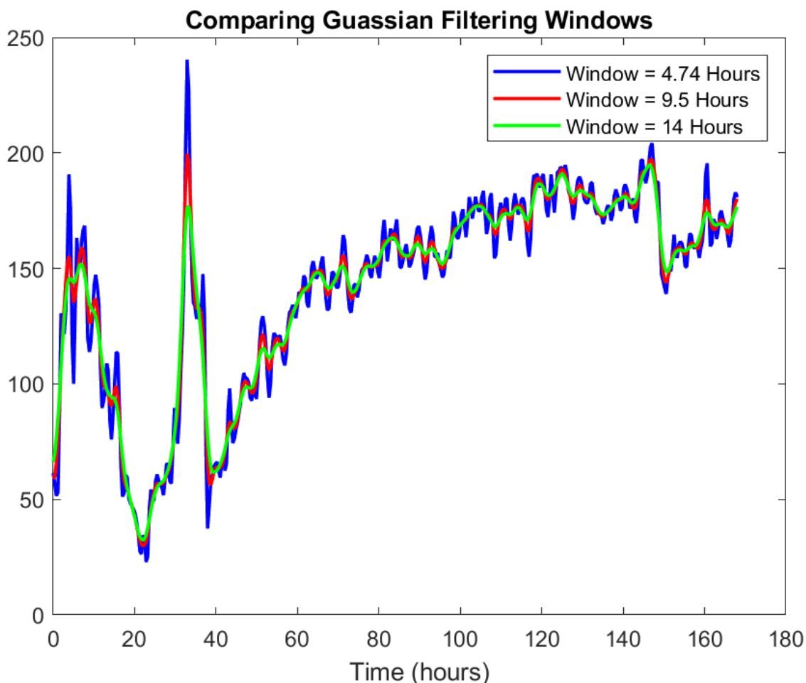
Fig. S6: Effect of Gaussian smoothing scales on Data. This representative p53 fluorescence trace taken over 168 hours following doxorubicin treatment, is shown under multiple Gaussian smoothing window sizes. Increasing the smoothing scale progressively suppresses transient peak features, including biologically relevant peaks at approximately 2 and 36 hours.
