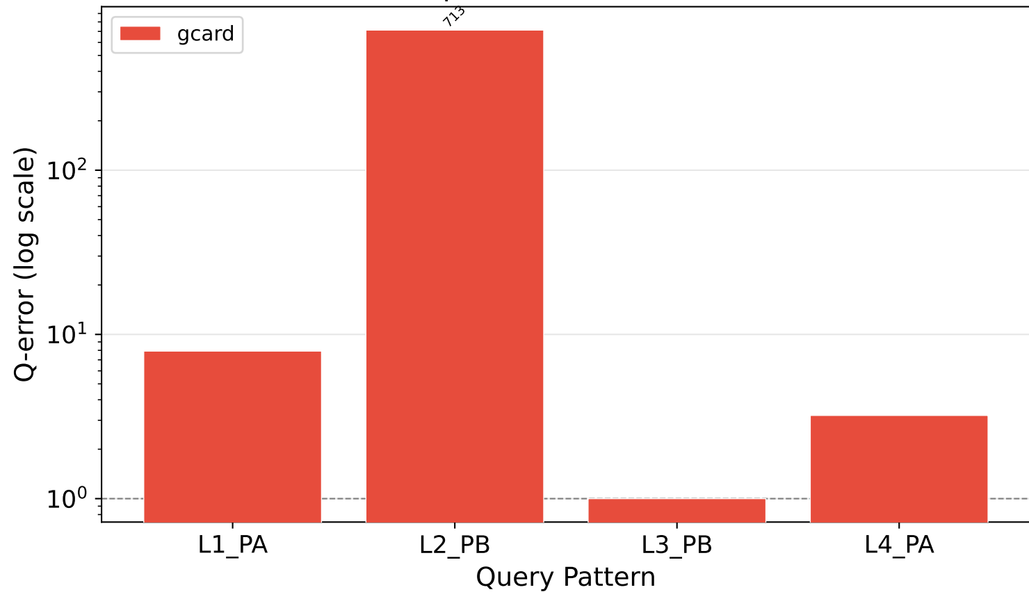
Q-error Comparison (With Predicates, SF1)
